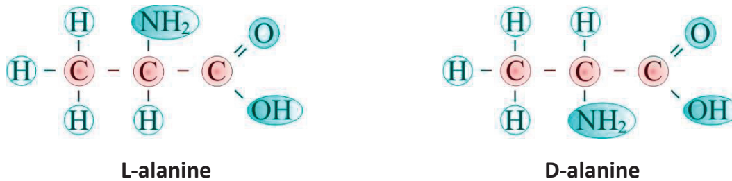
FIGURE 5.2 - The stereoisomers L and D of the amino acid alanine. Their spatial structures are non-superimposable images, similar to the right and left hands.
