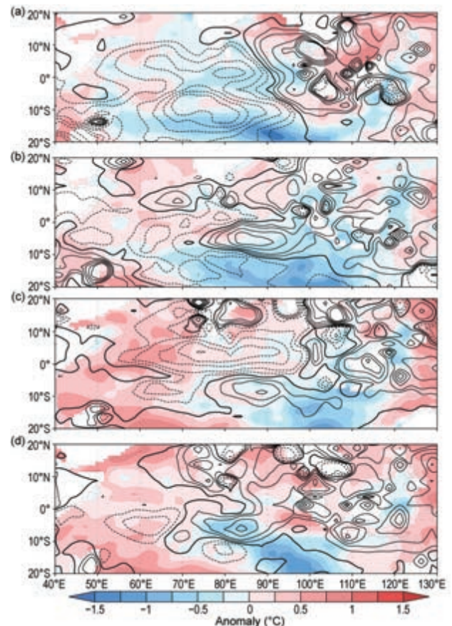
FIG. 4.41. SST ( ^{\circ}\text{C} ; colors) and precipitation (contoured at: 0, \pm 0.5 , \pm 1 , \pm 2 , \pm 3 , \pm 4 , and \pm 5 \text{ mm day}^{-1} ). Solid/dashed lines denote positive/negative values, and thick solid lines indicate the zero contour) anomalies during (a) Dec 2016–Feb 2017, (b) Mar–May 2017, (c) Jun–Aug 2017, and (d) Sep–Nov 2017. Anomalies were calculated relative to 1982–2017. [Sources: NOAA OISST (Reynolds et al. 2002) and monthly GPCP precipitation analysis (available at http://precip.gsfc.nasa.gov/ ).]
