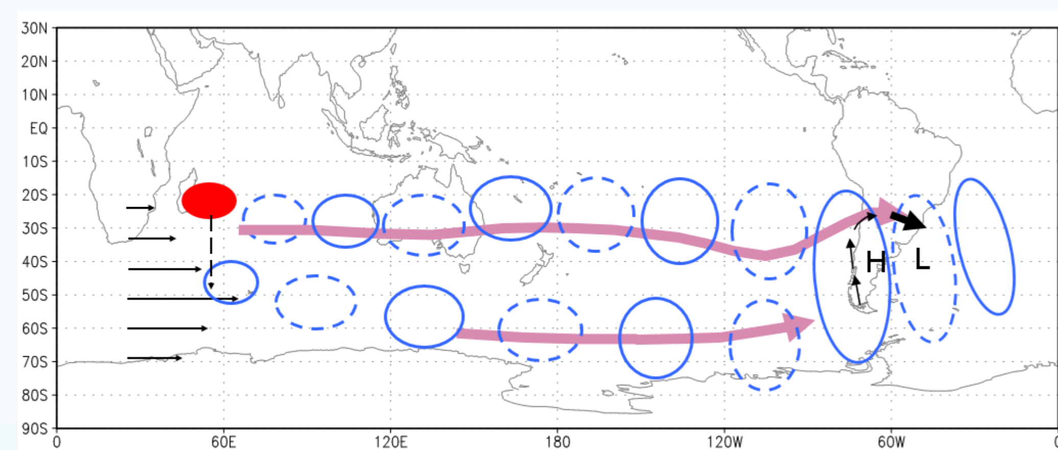
Figure 1: Conceptual diagram on the physical mechanisms that may favor high frequency occurrence of GF over PH.
