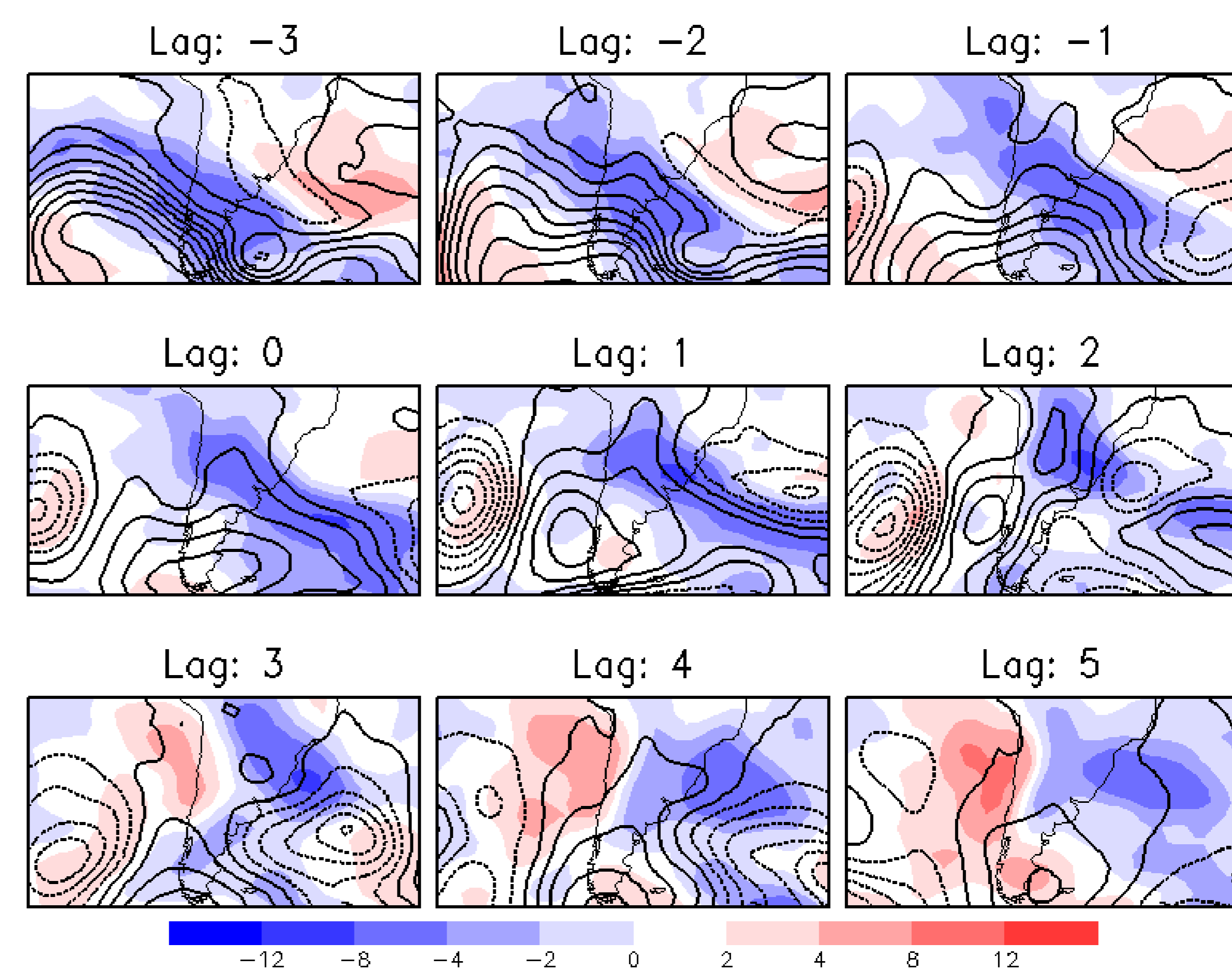
Figure 2: Geopotential height perturbations (contour) and temperature perturbations (shaded) at 850 hPa. Contour interval is 20 m.
