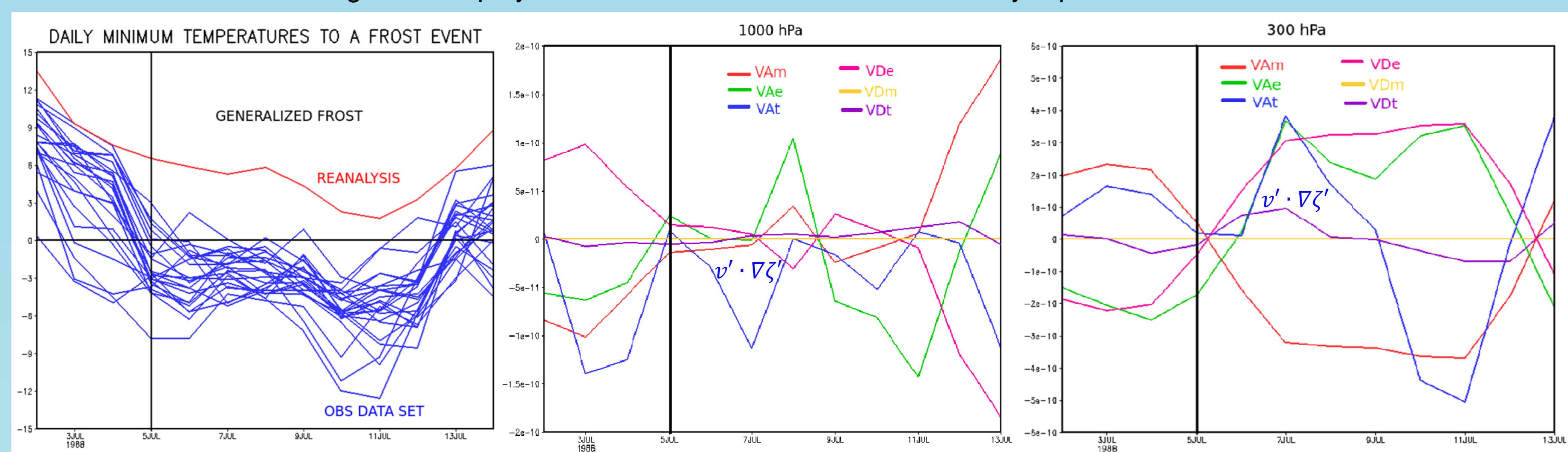
Figure 3: Observed daily minimum temperatures and vorticity equations terms to the very persistent 1988 GF event
