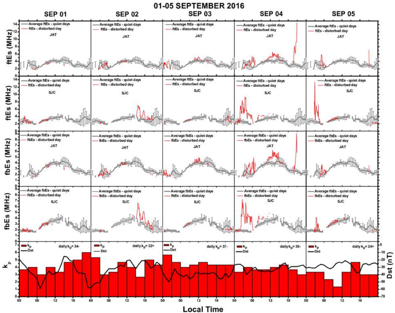
Figure 4. The two top panels show the mean quiet-time (gray lines) and storm-time (red lines) values of the top frequency ( f_t E_s ) reflected by the sporadic layers at JAT and SJC, respectively, during the moderately disturbed period of 1–5 September 2016. Similarly, in the middle panels is shown the blanketing frequency ( f_b E_s ) at JAT and SJC. The K_p and Dst values are shown in the bottom panel.
