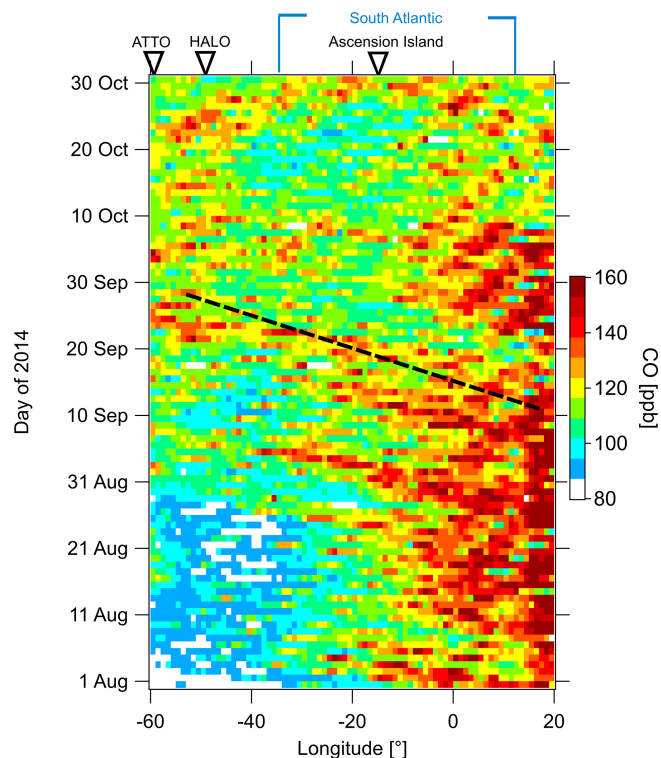
Figure 8. Hovmöller plot of the daily AIRS-derived carbon monoxide (400 to 600 hPa) distributed over the South Atlantic region ( 60^\circ \text{ W} to 20^\circ \text{ E} ) from August to October 2014, averaged over the latitudinal band of 10^\circ \text{ S} to 5^\circ \text{ N} , corresponding to the region of interest (ROI) highlighted in Fig. 7a 1 . Several events of transatlantic transport of aerosol from Africa towards South America can be identified. The black dashed line highlights a particularly strong plume originating around 10 September 2014 and arriving in the observational area of AC19 on 30 September.
