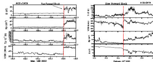
FIGURE 1 - Shocks profile of Fast Forward Shock on May 18th 2002, and of Slow Forward Shock on February 22nd 2000.
