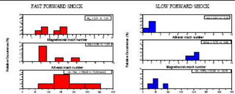
FIGURE 3 - Histograms comparing the fast and slow forward shock parameters: magnetosonic Mach numbers and shock speed to solar wind speed.
