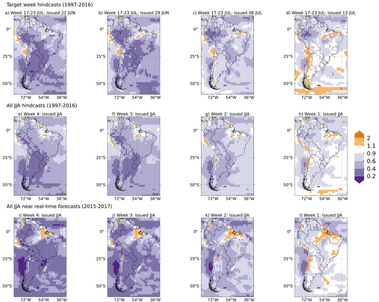
FIG. 5. Maps of the ratio of the predicted ECMWF ensemble mean temperature anomaly standard deviation and the observed temperature anomaly standard deviation for predictions produced from four to one week in advance (shown from left to right) for (a)–(d) the target week hindcast verification sampling strategy (20 samples), (e)–(h) the all-season hindcast verification sampling strategy (280 samples), and (i)–(l) the all-season real-time forecast verification sampling strategy (40 samples) described in the text.
