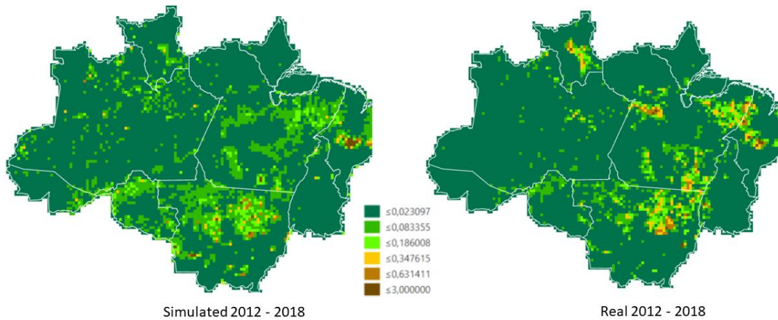
Figure 4.2 - Percentage of degradation in 25 x 25 Km 2 cells from 2012 to 2018 a) Simulated by LuccME, b) Real data.
