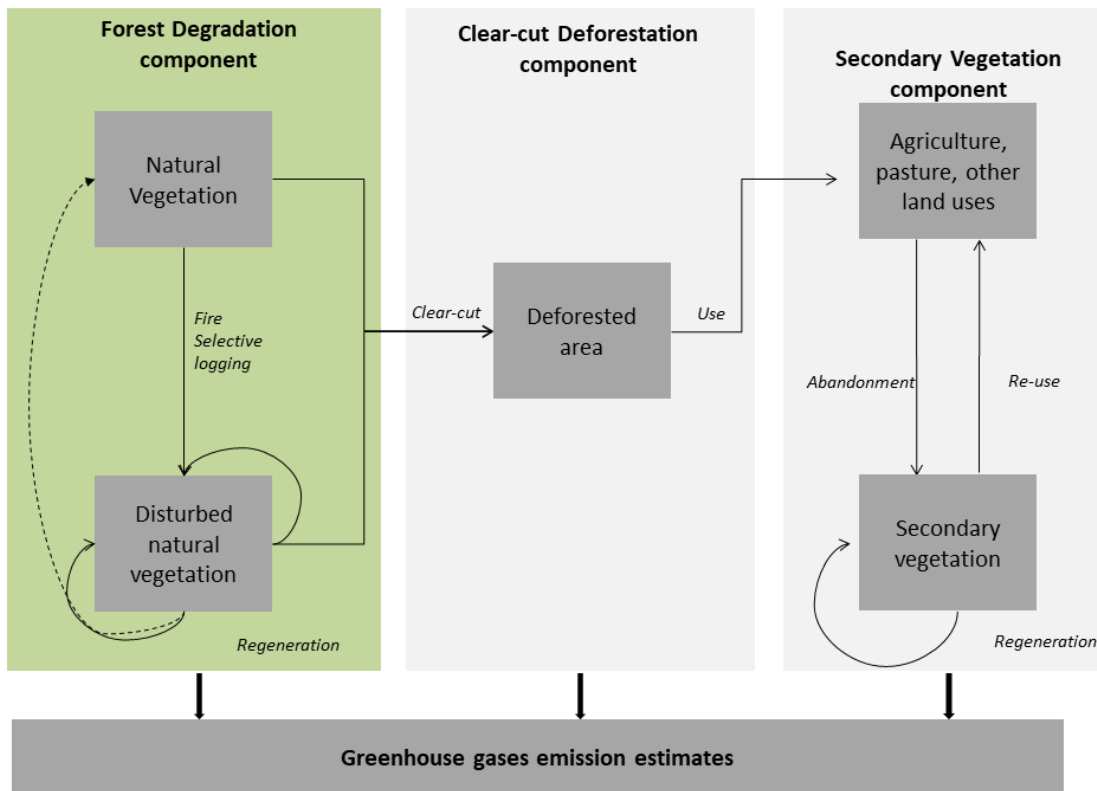
Figure 3.2 - INPE-EM model diagram.
