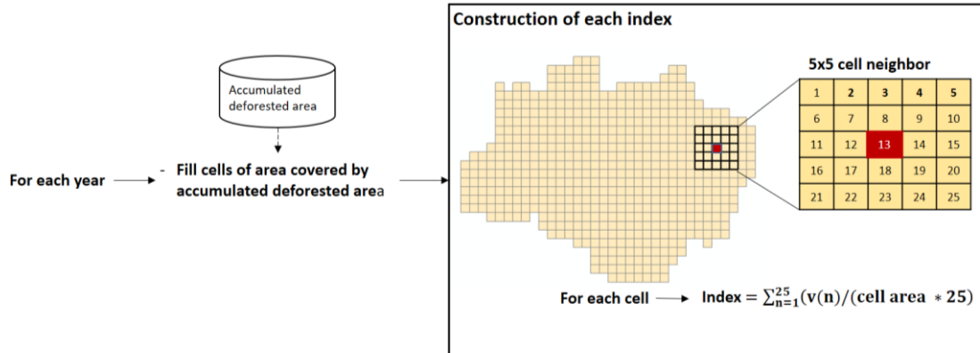
Figure 2.2 - Schematic graph of indicator construction.
