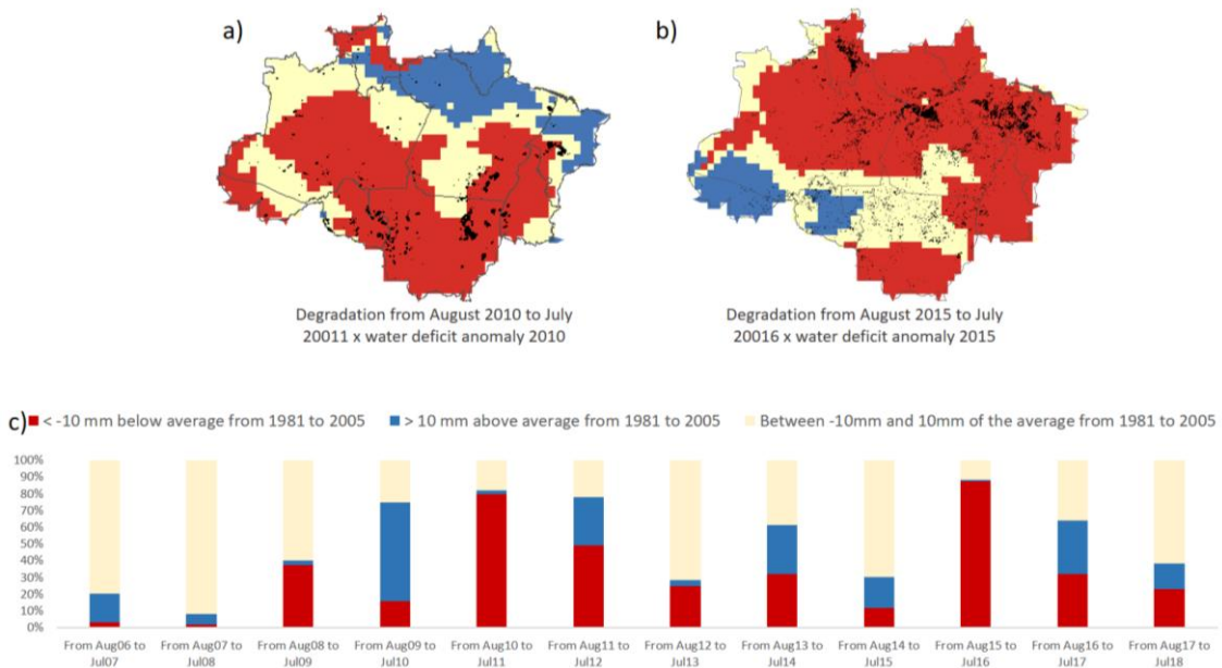
Figure 2.3 - Degradation area by water deficit anomaly indicator. a) Degradation from August 2010 to July 2011 x MCWD anomaly 2010 b) Degradation from August 2015 to July 2016 x MCWD anomaly 2015 c) Graph of degradation area by MCWD anomaly.
