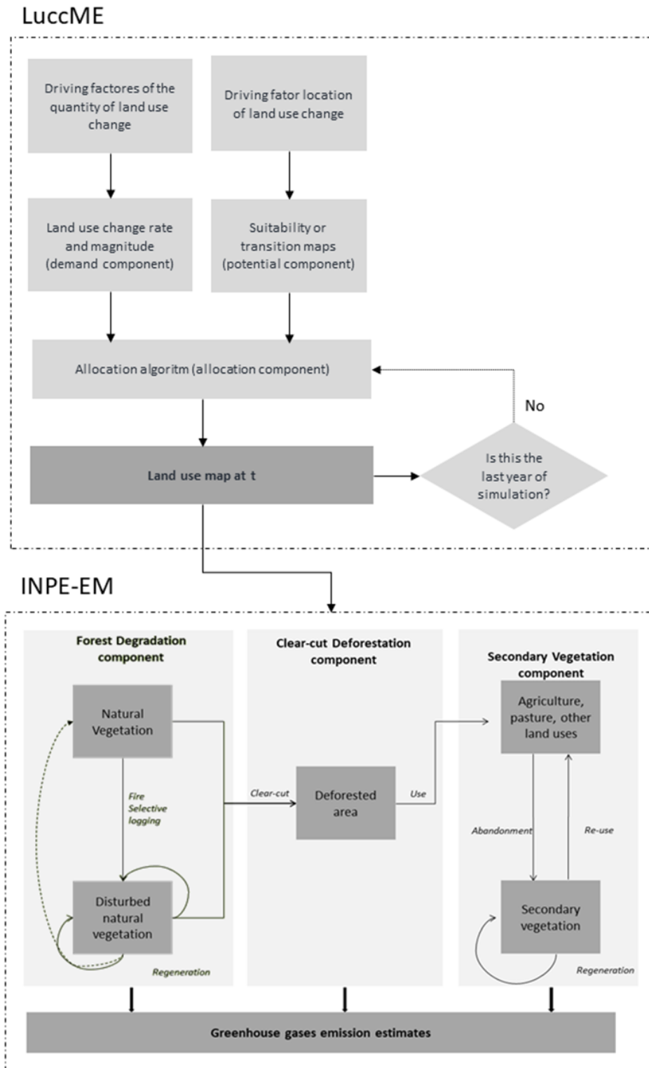
Figure 4.1 - LuccME modeling framework generates the annual land use maps, and INPE-EM represents the degraded forest dynamics and calculates the CO 2 emissions derived from this process.
