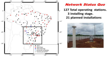
Fig 2: Stations for geodynamic monitoring installed by IBGE/INPE in the context of FAPESP thematic project
