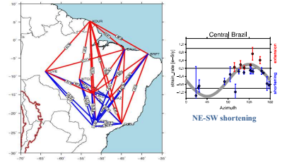
Fig 10: Strain Rates between all pairs of stations
