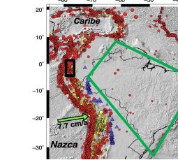
Fig 9: Stress patterns (stress inversions from foc. mechs.)
