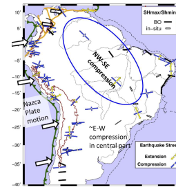
Fig 9: Stress patterns (stress inversions from foc. mechs.)
