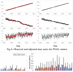
Fig 6: Observed and adjusted time series for POAL station
