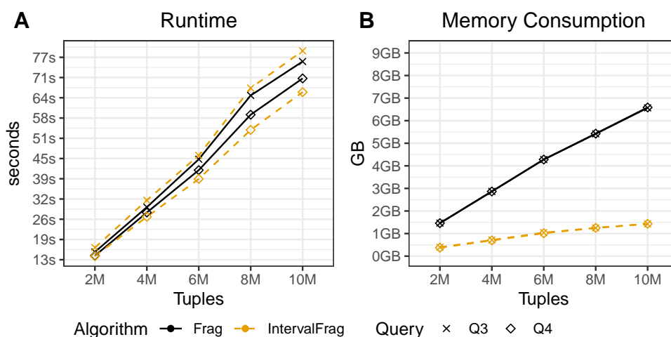
Figure 6.3 - IntervalFrag for Q3 and Q4.
