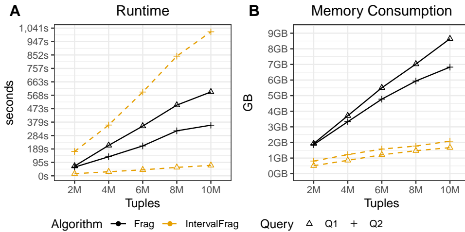
(A) Query response times of IntervalFrag and Frag-Cubing for queries Q1 and Q2 under the cube C0 . (B) Memory consumption of IntervalFrag and Frag-Cubing for queries Q1 and Q2 under the cube C0 .
