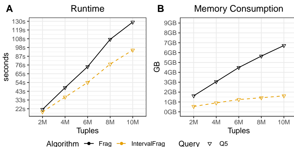
Figure 6.4 - IntervalFrag for Q5.
