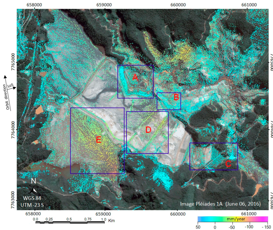
Figure 8. Ground displacement map in LoS of the Germano reservoir derived from the PSI analysis.
