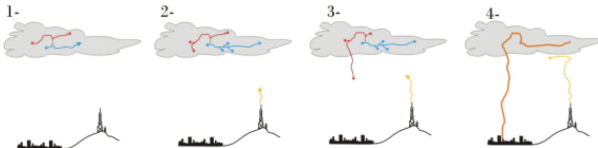
Fig 5. Leader over the tower is enough to trigger upward leader (IC or CG).
