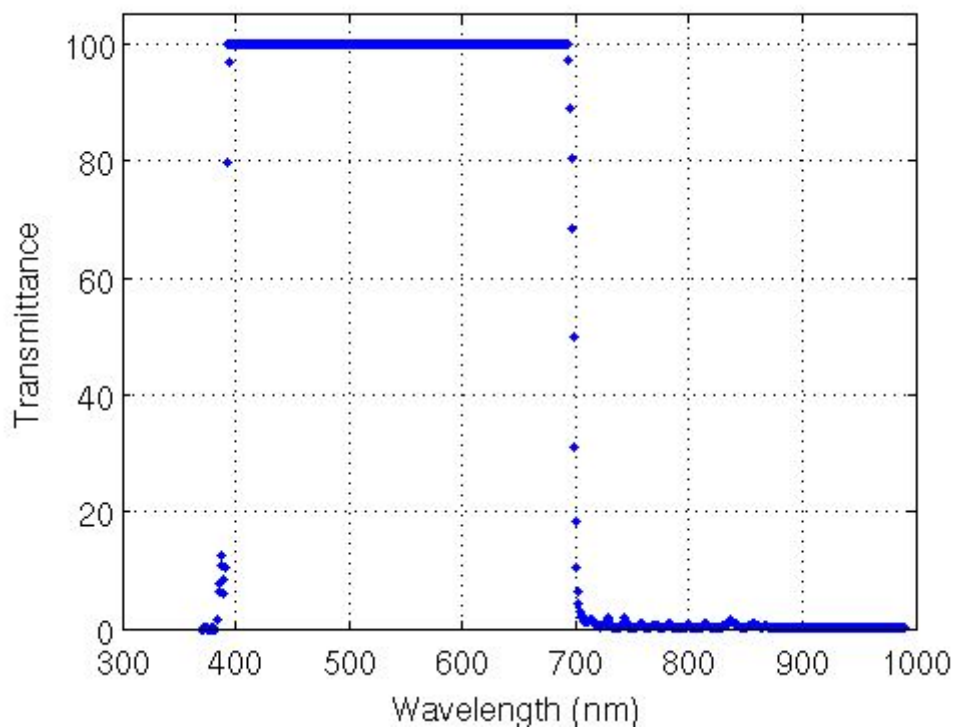
Figure 17. Transmittance measured in hot mirror filter 2. Lot # 7-4725
