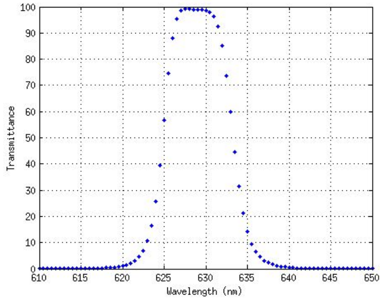
Figure 15. Transmittance measured in bandpass filter 9. Lot # 6-5997 Envelope 5
