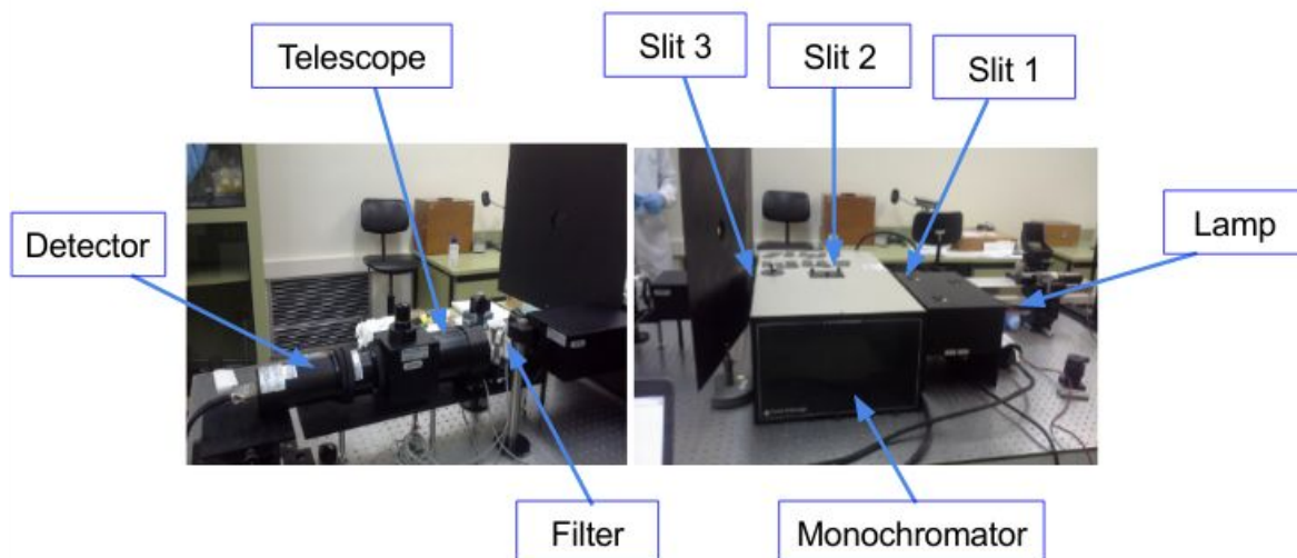
Figure 3. General view of the workbench and description of the components 8
