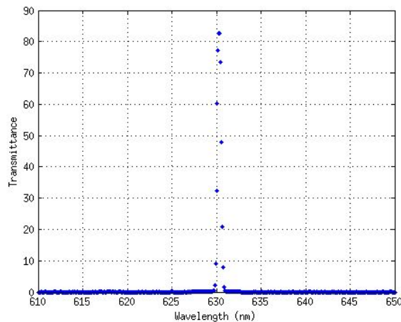
Figure 10. Transmittance measured in ultra narrow filter 6. Lot # 10-4080 Envelope 13 (first measure)
