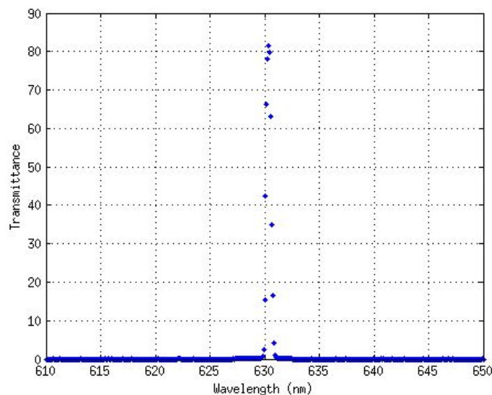
Figure 9. Transmittance measured in ultra narrow filter 5. Lot # 10-4080 Envelope 108
