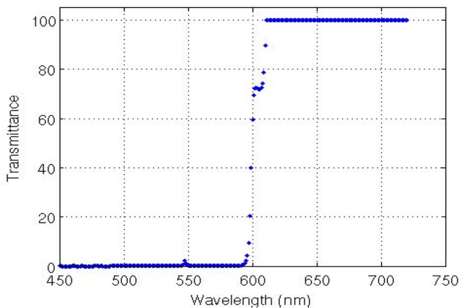
Figure 22. Transmittance measured in LP Dichroic filter 9. Lot # 7-4697
