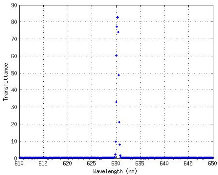
Figure 12. Transmittance measured in ultra narrow filter 6. Lot # 10-4080 Envelope 13 (third measure)
