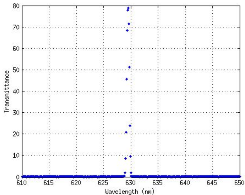
Figure 5. Transmittance measured in ultra narrow filter 1. Lot # 10-4080 Envelope 1
