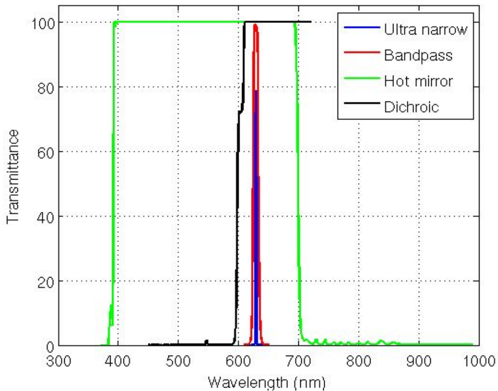
Figure 23. Ultra narrow, band pass, hot mirror, and dichroic filters.
