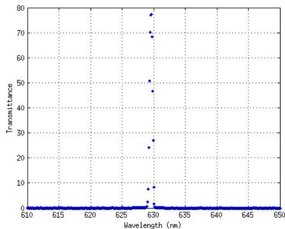
Figure 7. Transmittance measured in ultra narrow filter 3. Lot # 10-4080 Envelope 13
