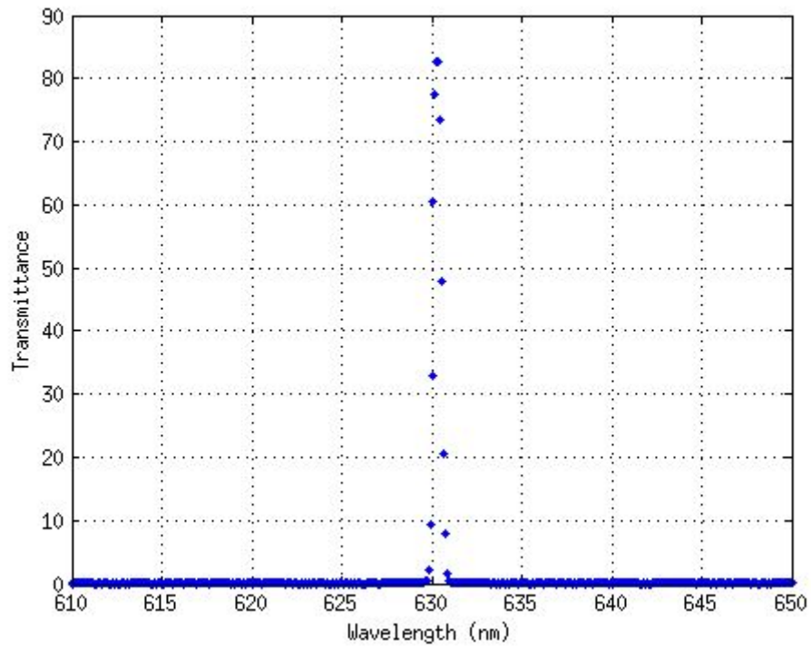
Figure 11. Transmittance measured in ultra narrow filter 6. Lot # 10-4080 Envelope 13 (second measure)
