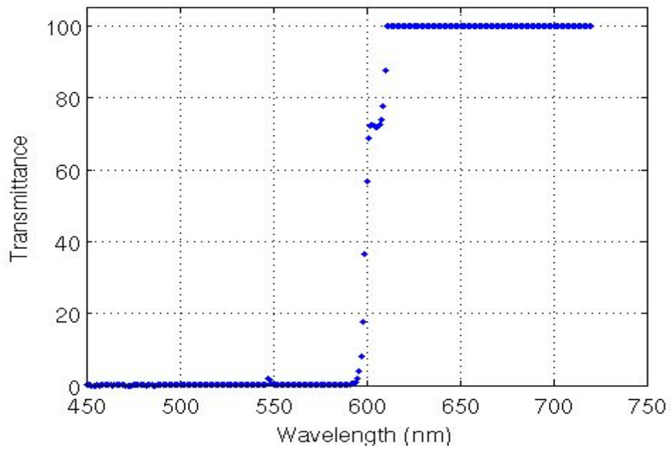
Figure 21. Transmittance measured in LP Dichroic filter 3. Lot # 7-4697 second measure
