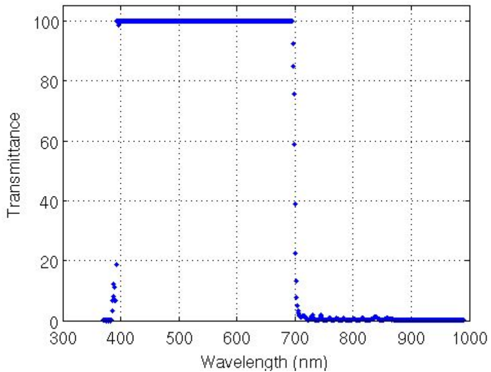
Figure 18. Transmittance measured in hot mirror filter 4. Lot # 7-4725
