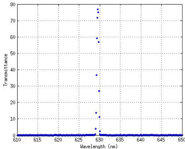
Figure 6. Transmittance measured in ultra narrow filter 2. Lot # 10-4080 Envelope 12
