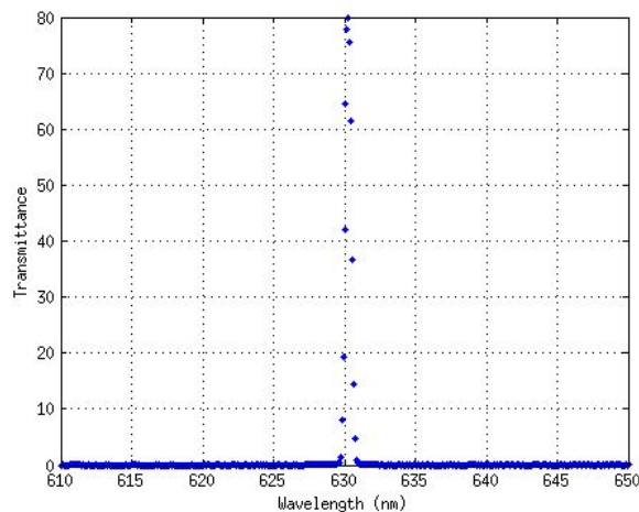
Figure 8. Transmittance measured in ultra narrow filter 4. Lot # 10-4080 Envelope 105
