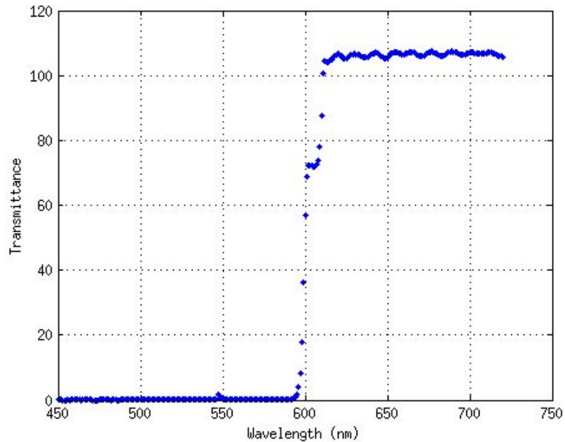
Figure 20. Transmittance measured in LP Dichroic filter 3. Lot # 7-4697
