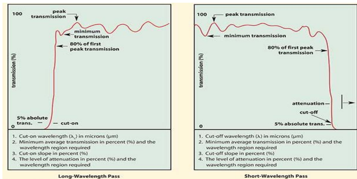
Figure 2. Long wavelength pass and short wavelength pass filters some characteristics 3 .
