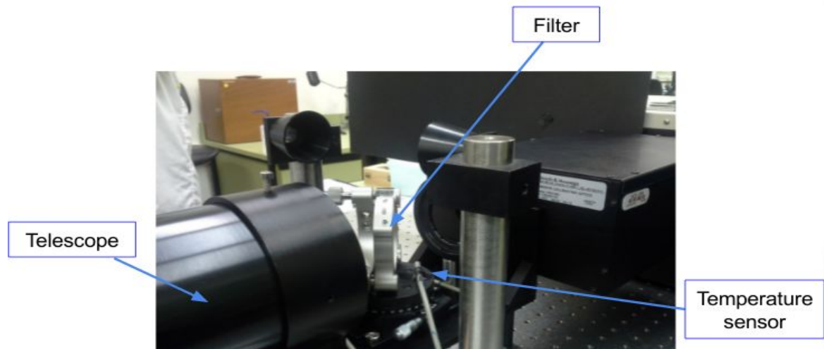
Figure 4. Highlight near to the filter setup
