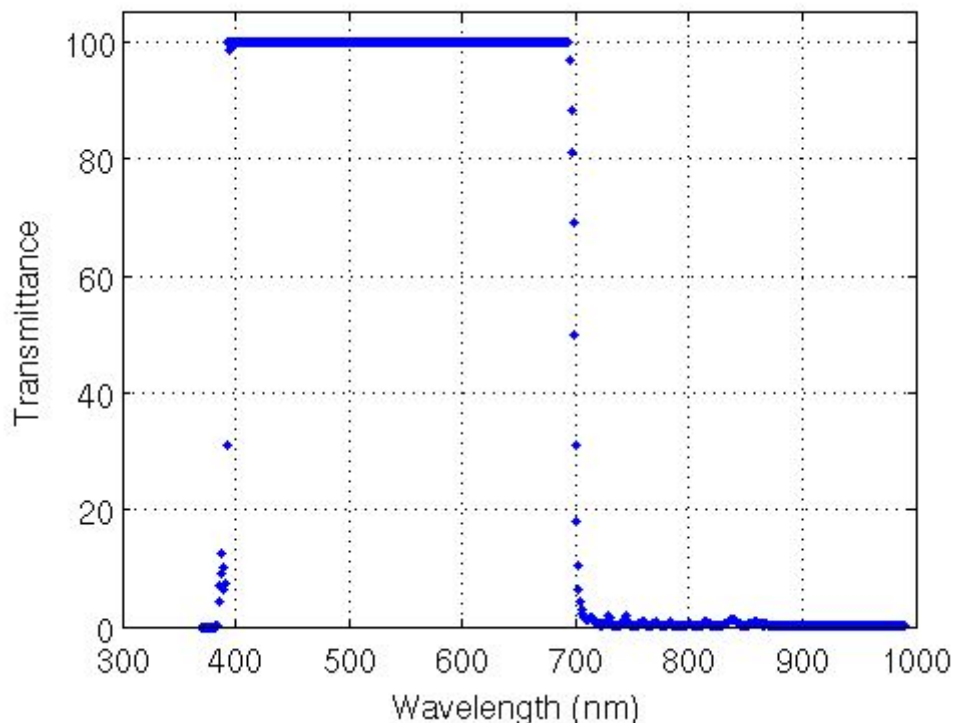
Figure 16. Transmittance measured in hot mirror filter 1. Lot # 7-4725
