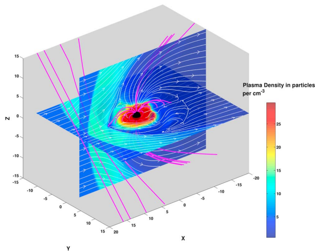
Figure 2. Global perspective of the interaction of the solar wind with the Earth's magnetosphere simulated by the Block-Adaptive-Tree-Solarwind-Roe-Upwind-Scheme code. The pink lines represent the IMF and dipolar magnetic field. The white solid lines with arrows represent velocity streamlines. Two cuts are shown, one at Y = 0 and the other at Z = 0 . The color code indicates the plasma density. The Sun is on the left, and the Earth is represented as a black sphere in the center.
