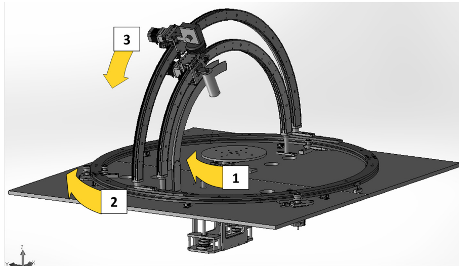
Figure 4 – Sequence of movements for the characterization of BRDF.
