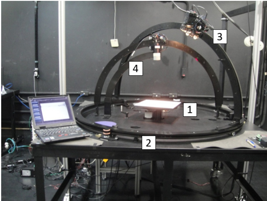
Figure 3 – Goniometer utilized during the in-lab BRDF determination.
