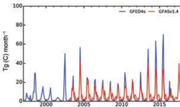
FIG. 2.68. Time series of fire activity during 1997–2017 in terms of carbon consumption ( \text{Tg month}^{-1} ) for North America.
