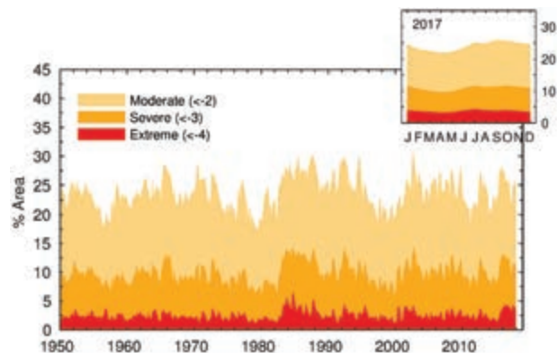
FIG. 2.31. Percentage of global land area (excluding ice sheets and deserts) with scPDSI indicating moderate (< -2), severe (< -3), and extreme (< -4) drought for each month of 1950–2017. Inset: each month of 2017.
