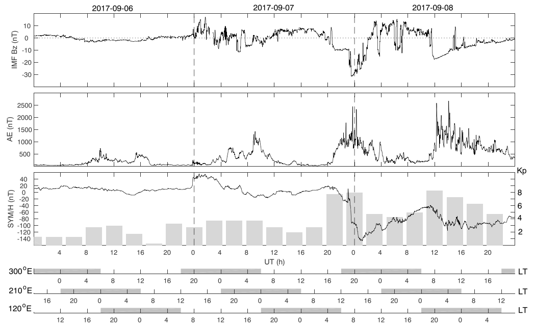
Figure 2. The interplanetary magnetic field B_z , AE, SYM/H, and K_p indexes during 6–8 September 2017. The axes in the bottom show the corresponding local time in the American (300°E), Pacific (210°E), and East Asian (120°E) sectors, respectively.
