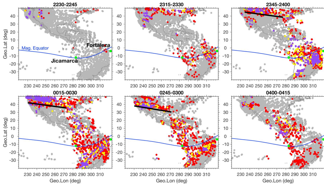
Figure 5. Rate of total electron content change index maps at selected time intervals (on 7–8 September) in the American sector. The green dots mark the locations of the two ionosondes. The superimposed black slant line marks the irregularity structure aligned along the northwest-southeast direction.
