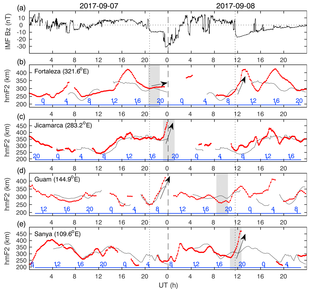
Figure 10. (a–e) The variations of interplanetary magnetic field B_z and of ionospheric hmF2 observed at Fortaleza, Jicamarca, Guam, and Sanya on 7–8 September 2017. The gray lines are geomagnetic quiet day (6 September 2017) values. The shaded region marks the sunset hours (1800–2000 LT).
