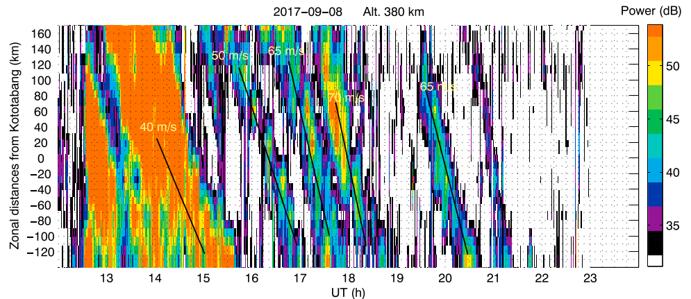
Figure 9. Echo intensity by the Kototabang radar 16-beam steering measurements at 380-km altitude during 1200–2300 UT on 8 September 2017, as a function of zonal distance (positive values represent the east) and time. The superimposed black slant line represents the slope of linear fitting employed for the calculation of zonal drift (from left to right: 40, 50, 65, 70, and 65 m/s westward).
