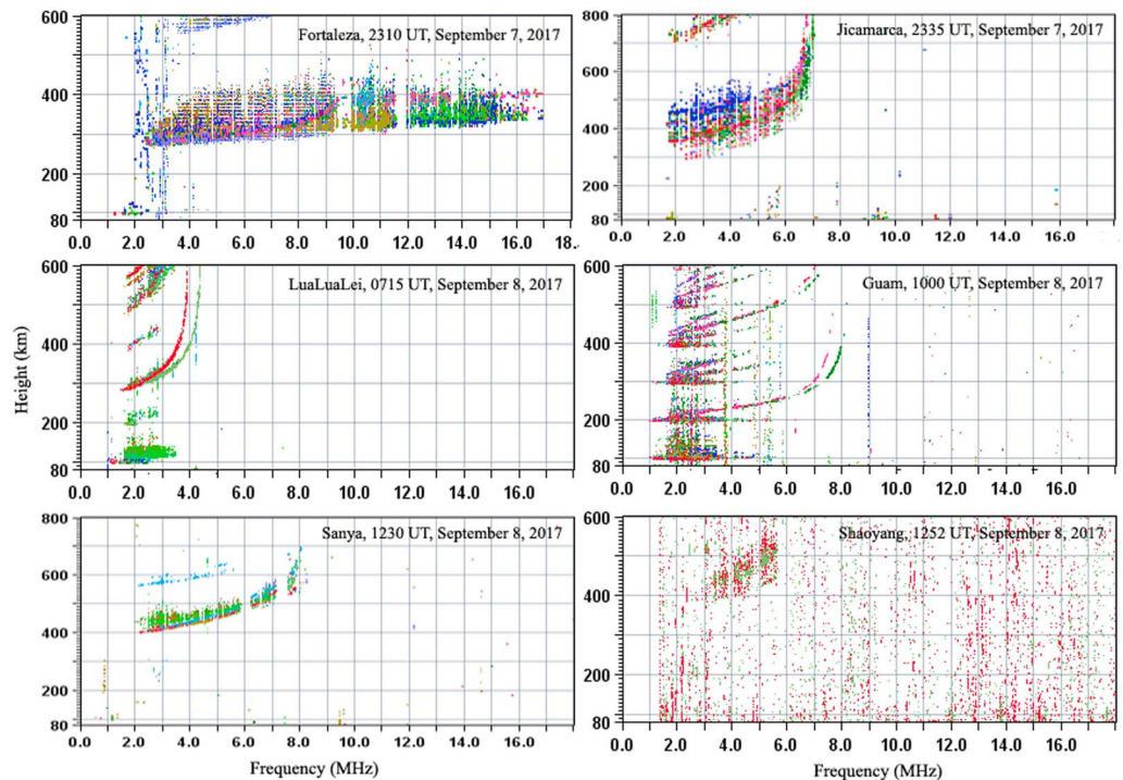
Figure 4. Selected ionograms showing the presence/absence of equatorial plasmabubbles over Fortaleza, Jicamarca, Lualualei, Guam, Sanya, and Shaoyang.
