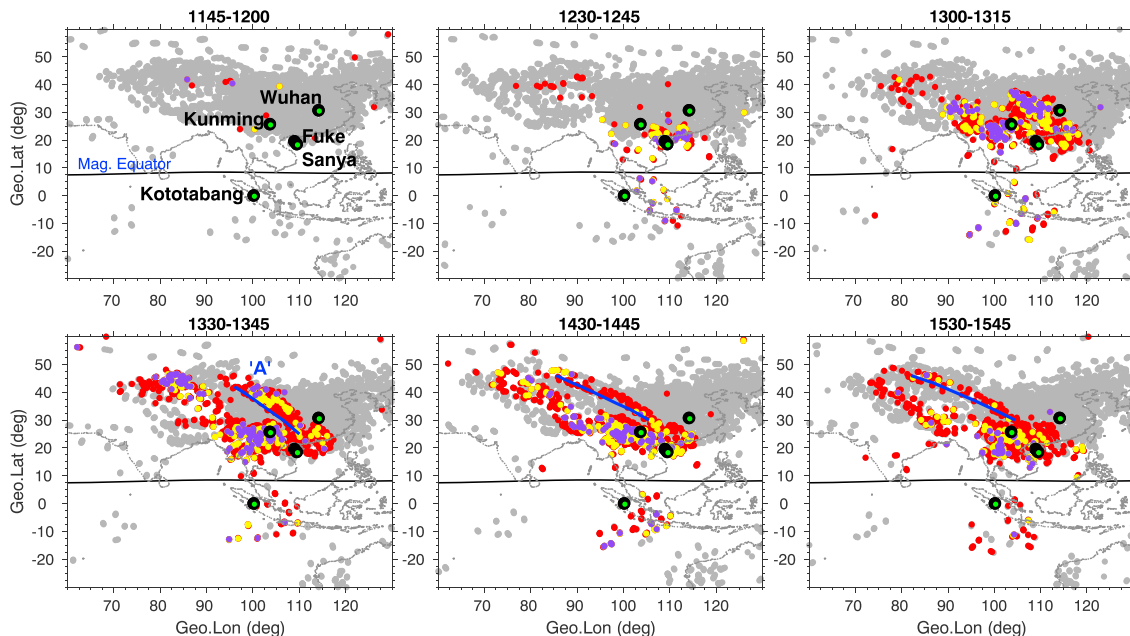
Figure 6. Rate of total electron content change index maps at selected time intervals (on 8 September) in the Asian sector. The black circles with green dots mark the locations of the very high frequency radars. The superimposed blue curve in the bottom panel represents the west wall of the west-tilted structure “A.”
