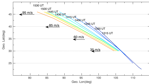
Figure 7. The positions of the west-tilted structure “A” (shown in Figure 6) at different time intervals. The drift velocities at four selected latitudes (30°N, 35°N, 40°N, 45°N) were estimated, about 35, 60, 85, and 95 m/s, respectively.
