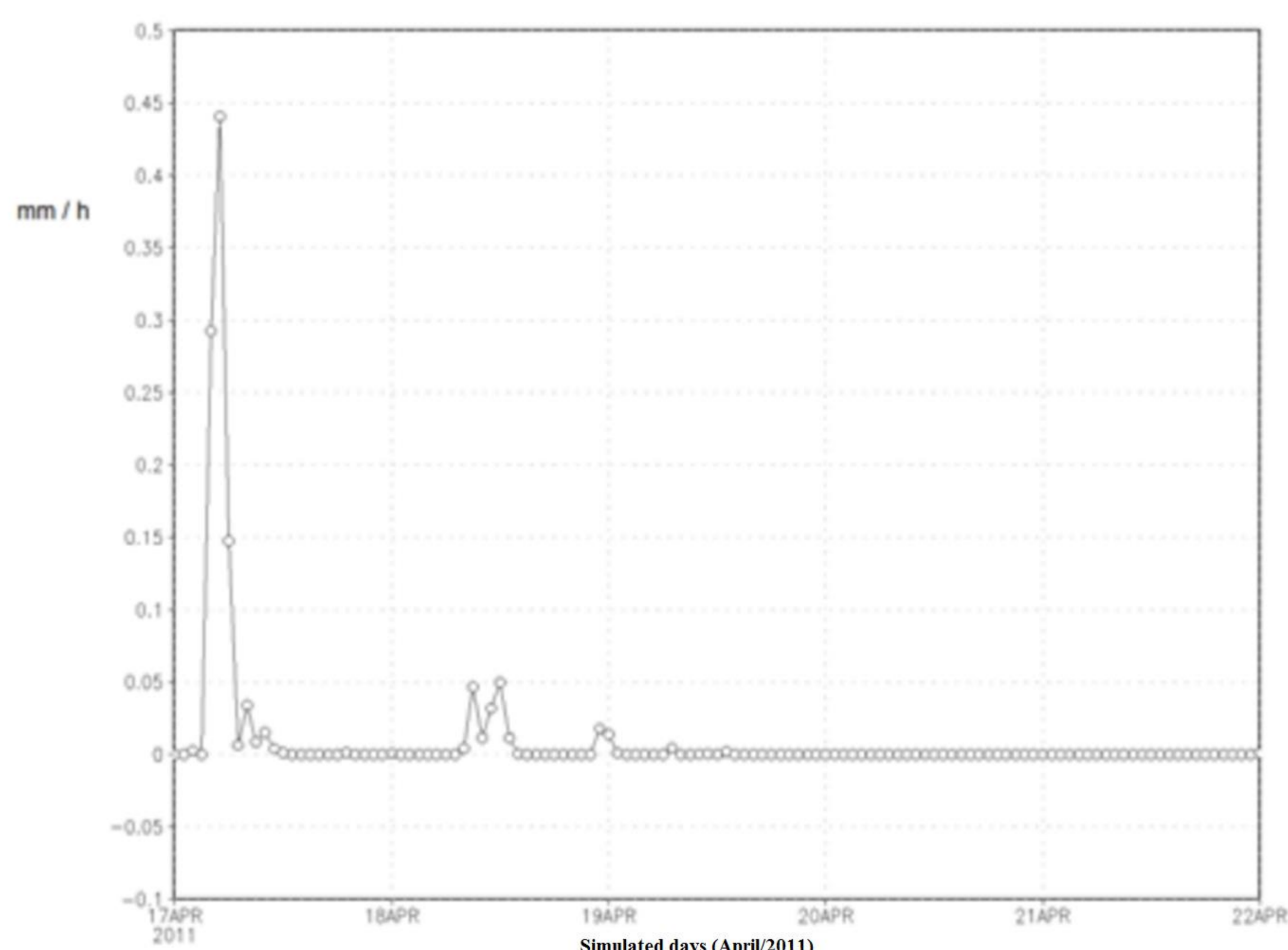
Figure 1 -Hourly precipitation simulated from April 17 to 22, 2011
