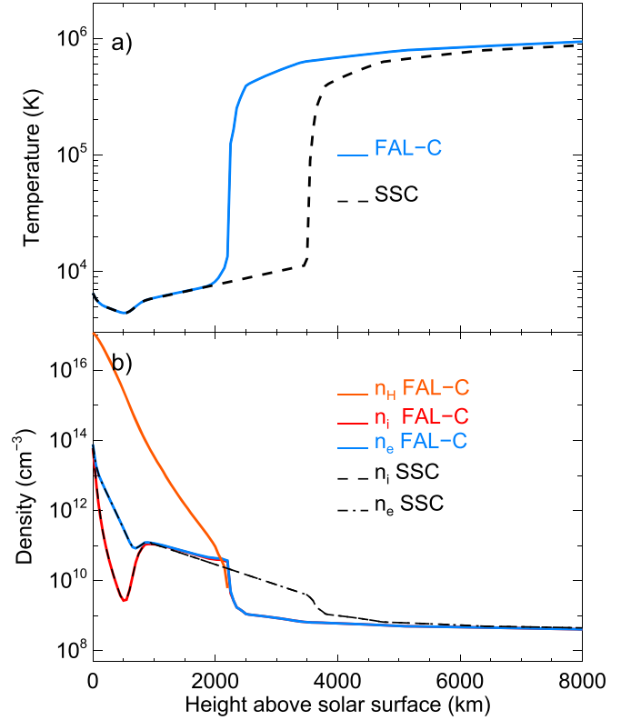
Figure 3. (a) Temperature and (b) densities ( n_e , n_i , and n_{\text{H}} ) distributions for the FAL-C and SSC atmospheric models.
