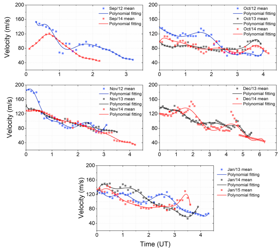
Figure 6. Mean (scatter) and polynomial fitting (curve) from equatorial plasma bubble velocities to each group of specific month.
