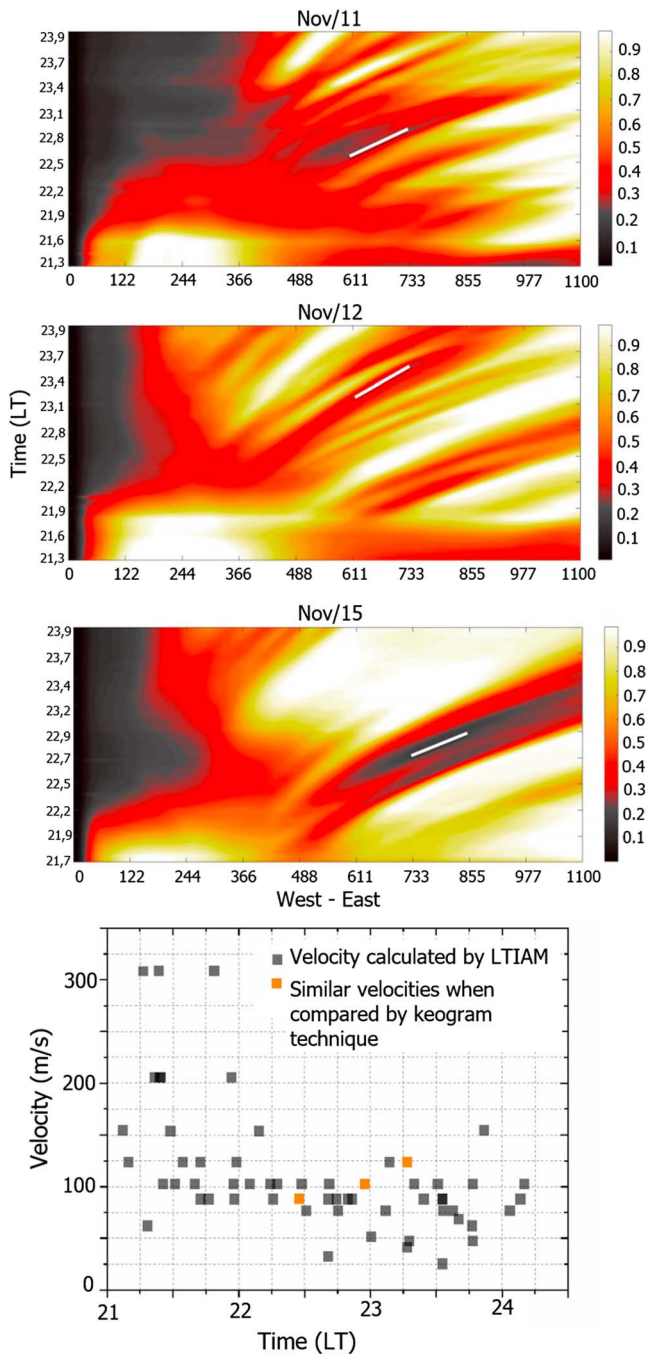
Figure 7. Keograms and scatter plot (bottom panel) from equatorial plasma bubble velocities comparing results from Long-Term Ionospheric Anomaly Monitoring and optical technique. The regions of equatorial plasma bubbles are represented by dark colors in keograms. The solid white line represents an interval that is possible to infer velocity value from coordinates of the final and start points. The orange squares in scatter plot represent similar velocities obtained by Long-Term Ionospheric Anomaly Monitoring in comparison to keogram technique.
