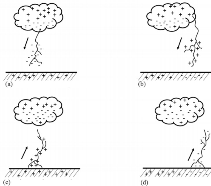
Figure 2.11 – Illustration showing the different types of CG flashes. (a) Negative downward flash; (b) Positive downward flash; (c) Negative upward flash; and (d) Positive upward flash.
