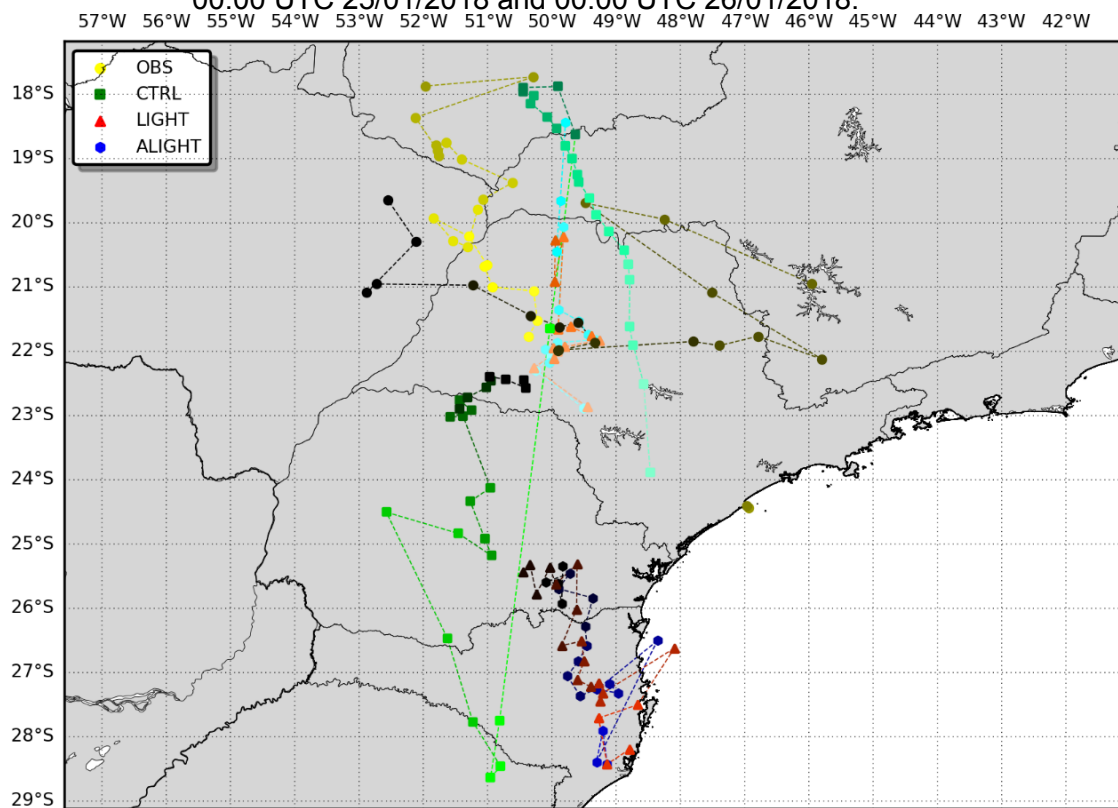
Figure 4.33 – Representation of the location of the center of mass calculated based on the Reflectivity field in 3 km simulated by the experiments and of the geometric center based on lightning detections for the period between 00:00 UTC 25/01/2018 and 00:00 UTC 26/01/2018.
