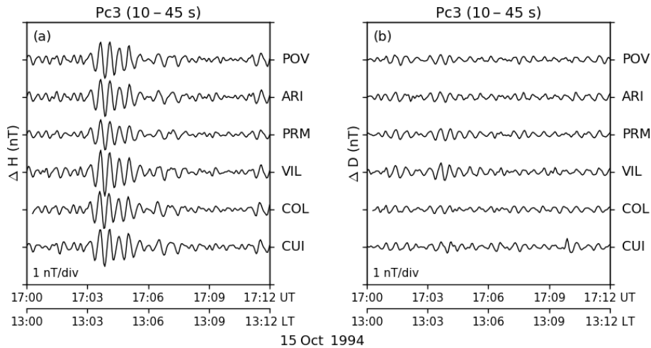
Figure 3. Band-pass-filtered geomagnetic variations ( H and D components) in the Pc3 interval (10–45 s), shortly after noon on 15 October 1994. A Pc3 event starting at \sim 13:03 LT is observed.
