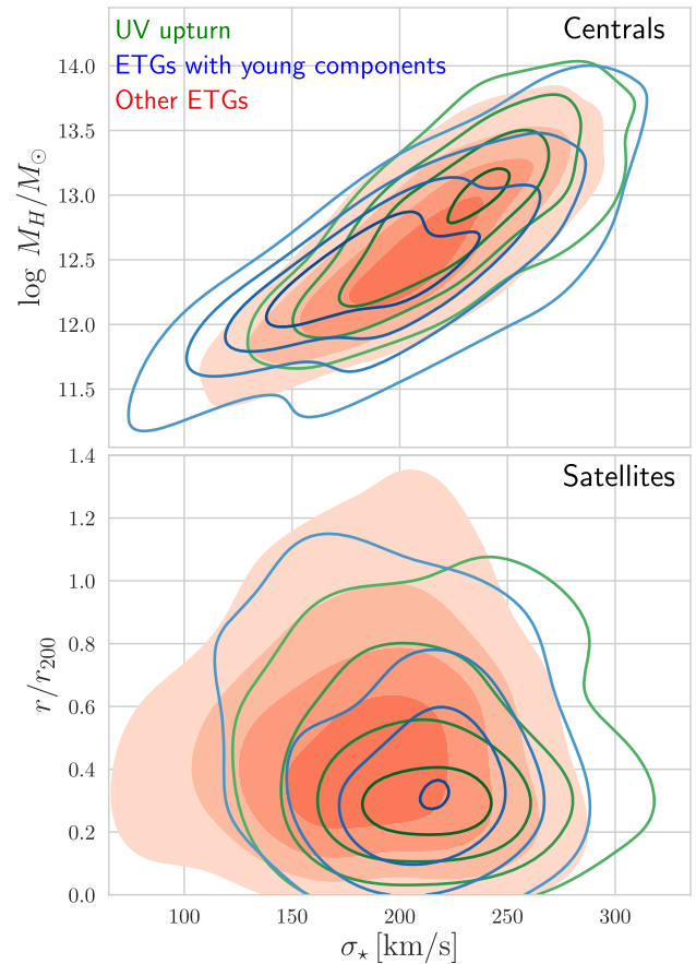
Figure 10. Top: Stellar velocity dispersion ( \sigma_* ) against halo mass ( \log M_H ) for central galaxies. Bottom: \sigma_* against the projected distance to the luminosity-weighted centre of the dark matter halo (normalized by r_{200} ) for satellite galaxies. Blue contours correspond to ETGs with young components, green contours correspond to UV upturn galaxies, and filled red contours in the background show the distribution for other ETGs. Contours trace a kernel density estimates calculated using a Gaussian kernel.
