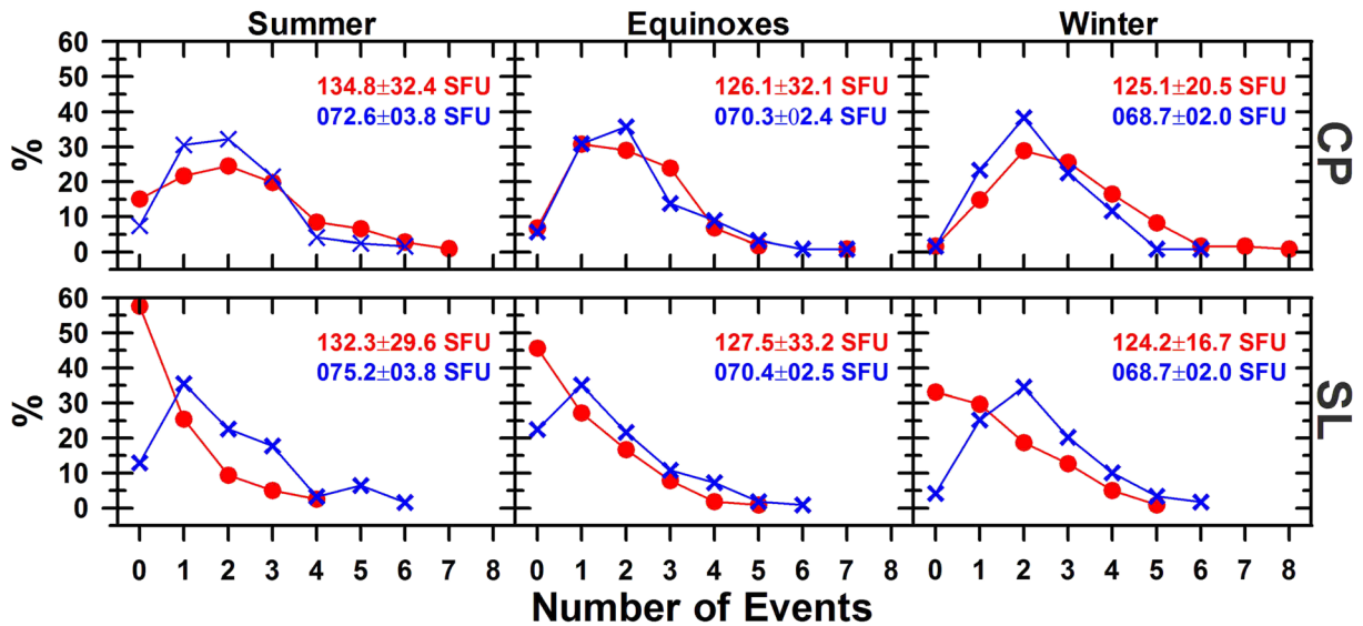
Figure 3. Percentage of occurrence of the number of events per day for December solstice, equinoxes, and June solstice (panels from left to right, respectively) over Cachoeira Paulista and São Luís (upper and bottom blocks, respectively). The red profiles represent the year 2003, while the blue ones the year 2009. Following the same color representation, each panel displays the average of solar flux as well as its standard deviation for each period in solar flux unit (1 SFU = 10^{-22} Wm -2 Hz -1 ).
