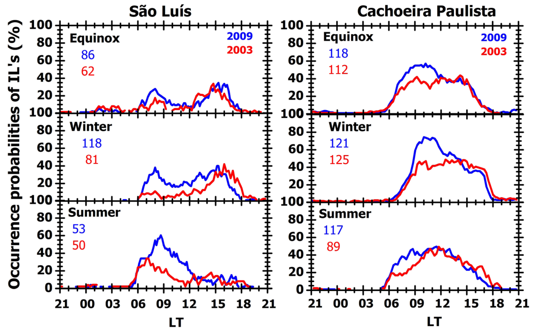
Figure 6. Occurrence probability of the intermediate layer events over SL (left) and CP (right) during 2009 (blue lines) and 2003 (red lines). Only the layers above 130 km were considered in this statistical analysis. The number of days with IL events used in the occurrence percentage calculation is indicated in each panel.
