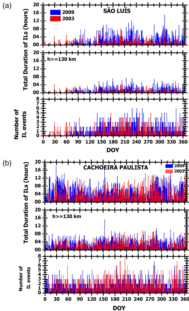
Figure 2. (a) Intermediate descending layers duration for different ranges of altitude (from top to bottom, first and second panel) and number of events over SL (third panel) during 2003 (red color) and 2009 (blue color). (b) Same as Part (a), but for CP.
