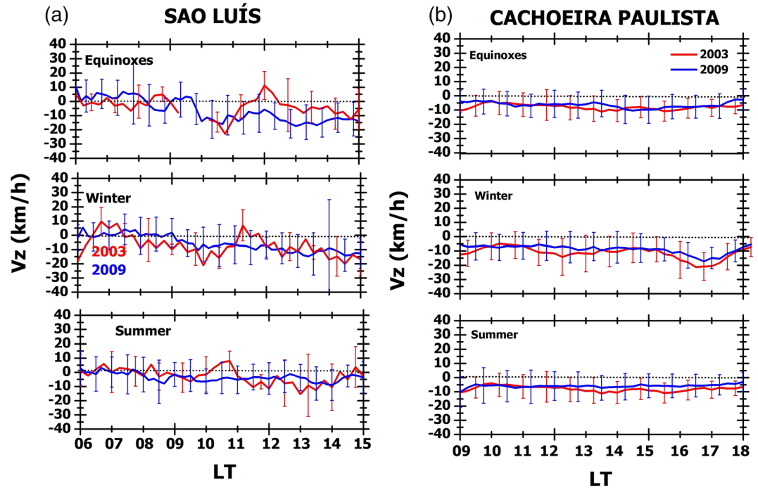
Figure 7. (a) Mean IL's vertical velocity ( V_z ) over SL for equinoxes, winter, and summer during 2003 (red line) and 2009 (blue line). (b) The same, but for CP. For a better visualization, the standard deviation shown in each panel was divided by a factor of 3.
