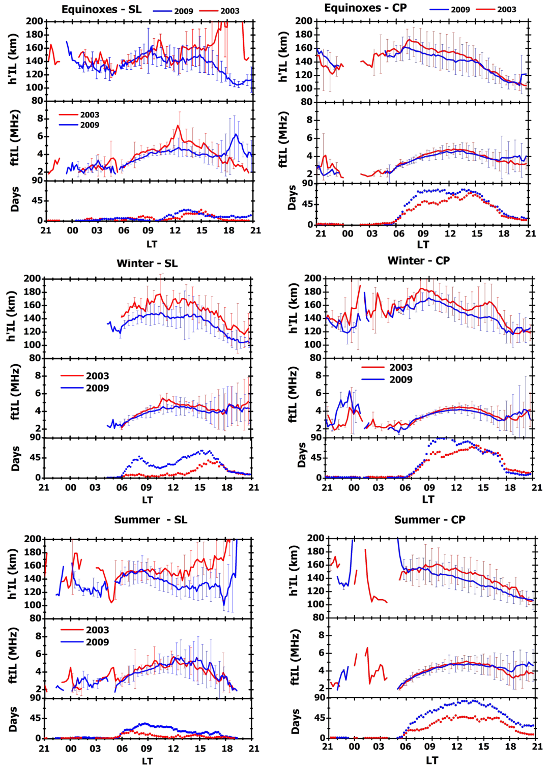
Figure 4. Local time variation of h'IL and ftIL from SL (left panels) and CP (right panels) for low and high solar activity periods (blue and red, respectively) for different seasons. The vertical bars represent the standard deviation. The bottom smaller panel of each plot shows the number of occurrences per local time.
