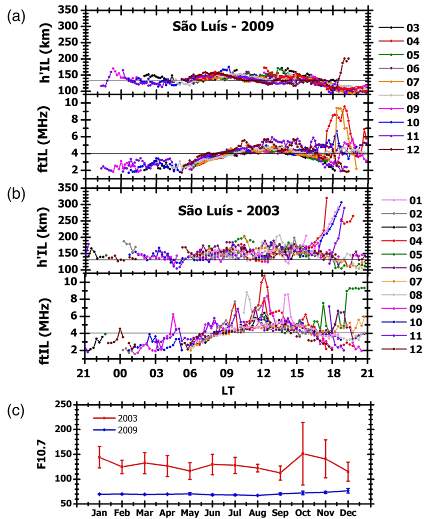
Figure 5. Monthly mean values of h'IL and ftIL over SL during (a) 2009 and (b) 2003. (c) The monthly mean F10.7 cm index (SFU) for 2009 (blue) and 2003 (red).
