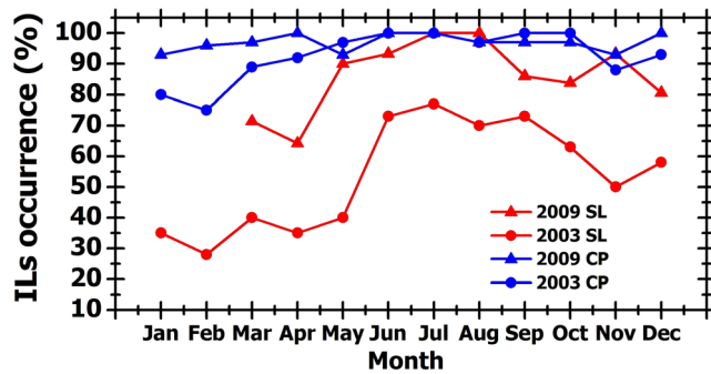
Figure 1. Intermediate descending layers' occurrence over SL (red lines) and CP (blue lines) during 2003 (circles) and 2009 (triangles).
