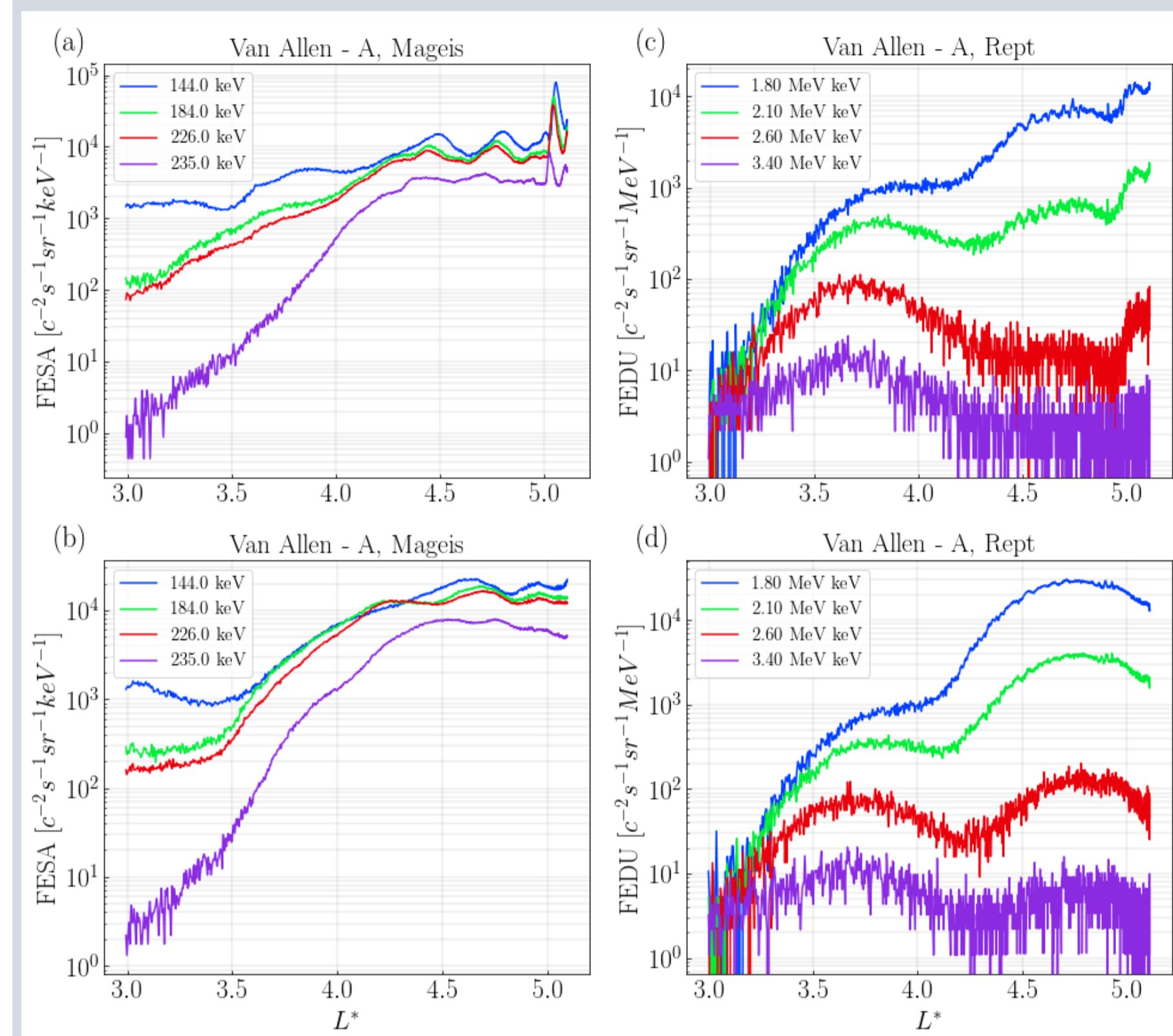
Figure: Low and high energy electrons flux density, corresponding to the second and third orbit in 09 February 2014.
