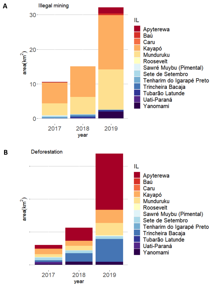
Figure 3.2 - Illegal mining and deforestation within indigenous lands in the Legal Amazon between 2017–2019. Illegal mining areas detected by DETER (A), deforested areas detected by PRODES (B).
