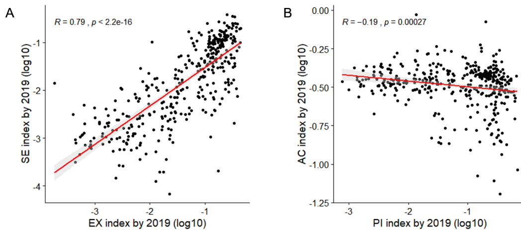
Figure 4.4 - Scatter plot of the final indexes of Exposure and Sensitivity (A), and Potential Impact and Adaptive Capacity (B). The indexes are displayed on a logarithmic scale. Indigenous lands are represented as points.
