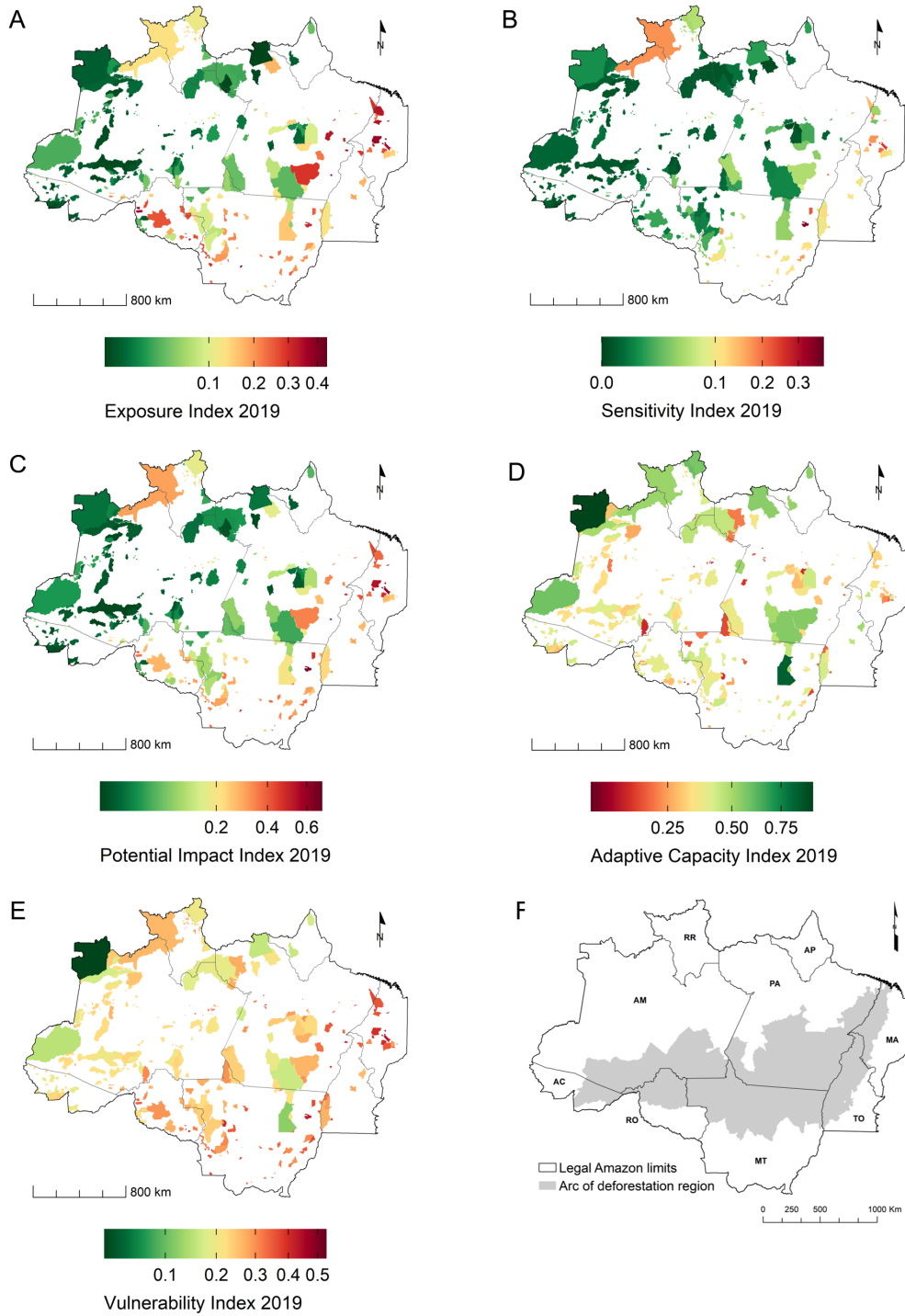
Figure 4.3 - Final indexes of Exposure (A), Sensitivity (B), Potential Impact (C), Adaptive Capacity (D), and Vulnerability (E) by 2019 of the Amazonian Indigenous Lands. Limits of the regions of the Legal Amazon and the arc of deforestation (F). The maps are displayed on a quadratic scale.
