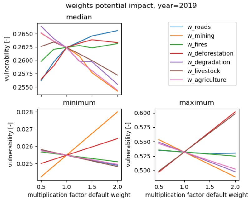
Figure 4.6 - The OAT sensitivity analysis results for the weights of the Potential Impact indicators (i.e. EX and SE indexes). The graphs show the influence of changes in the weights of the indicators on the median, the maximum and minimum value of the Vulnerability index.
