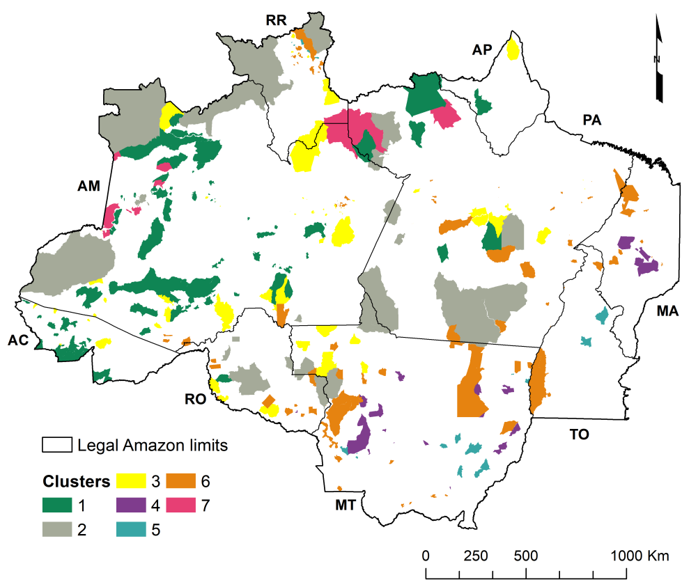
Figure 2.5 - Final clusters of Indigenous Lands according to the set of common environmental threats inside and outside these territories.
