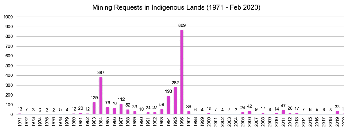
Figure A.2 - Mining requests in Indigenous Lands in the Amazon between 1971–Feb 2020.
