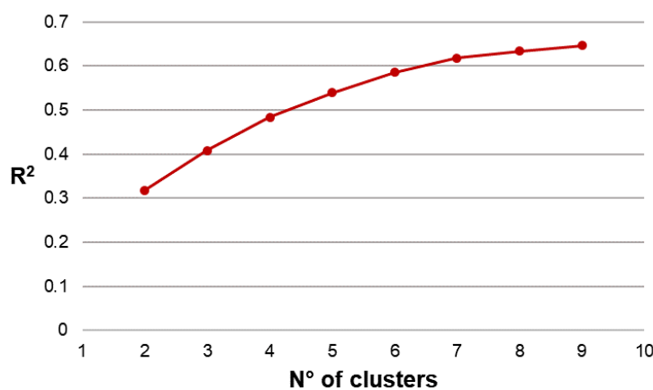
Figure 2.4 - Coefficient of determination of the number of clusters.
