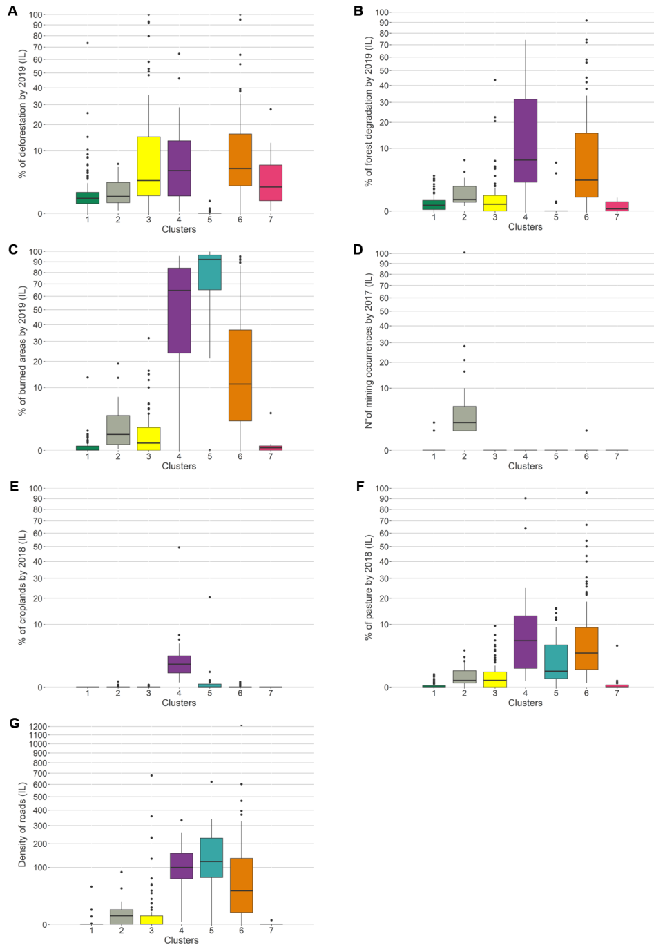
Figure 2.7 - Boxplots of environmental threats within Indigenous Lands (IL). Accumulated deforestation by 2019 (%) (A); Accumulated forest degradation by 2019 (%) (B); Accumulated burned areas by 2019 (C); Number of mining occurrences (D); Croplands by 2018 (%) (E); Pasture by 2018 (%) (F); Roads network density (km/km 2 ) (G). The axes increase quadratically to improve the visibility of differences. The upper and lower whiskers correspond to the first and third quartiles, and the line inside the box represents the median. Data beyond the end of the whiskers are outliers and plotted as points.
