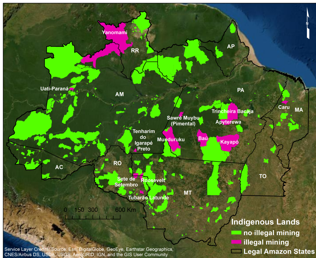
Figure 3.1 - Indigenous lands with illegal mining detected by DETER between 2017–2019. In white are indicate the names of the indigenous lands with illegal mining and the abbreviations of the states of the Legal Amazon region.
