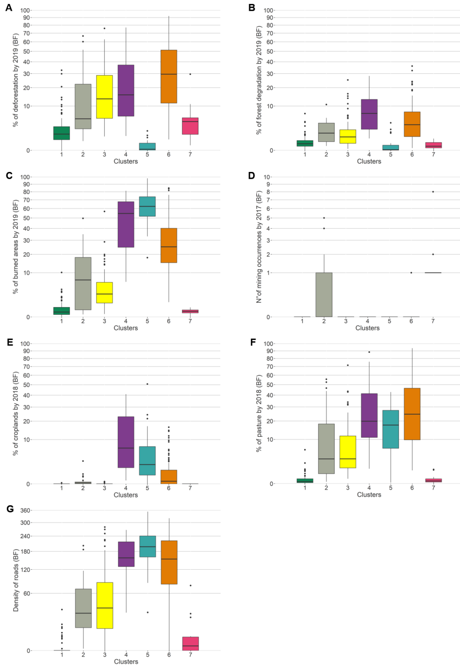
Figure 2.8 - Boxplots of environmental threats in the buffer zone (BF) of Indigenous Lands. Accumulated deforestation by 2019 (%) (A); Accumulated forest degradation by 2019 (%) (B); Accumulated burned areas by 2019 (C); Number of mining occurrences (D); Croplands by 2018 (%) (E); Pasture by 2018 (%) (F); Roads network density (km/km 2 ) (G). The axes increase quadratically to improve the visibility of differences. The upper and lower whiskers correspond to the first and third quartiles, and the line inside the box represents the median. Data beyond the end of the whiskers are outliers and plotted as points.
