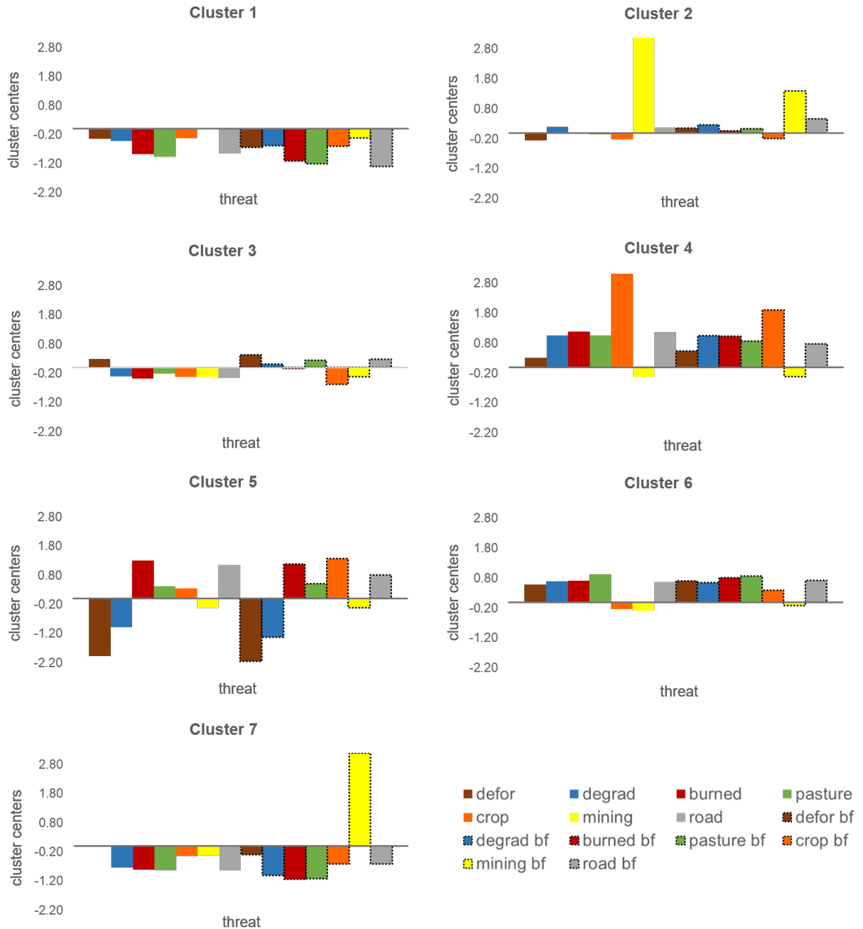
Figure A.1 - Bar charts of the clusters of Indigenous Lands. The values were plotted to represent the final cluster centers for each threat. Environmental threats within the Indigenous Land are plotted on the left, while threats in the Buffer Zone are plotted on the right with the dashed border. Threats in the buffer zone are identified by the abbreviation 'bf'. 'Defor' is an abbreviation for deforestation and 'degrad' for forest degradation. The central axis delimits the mean.
