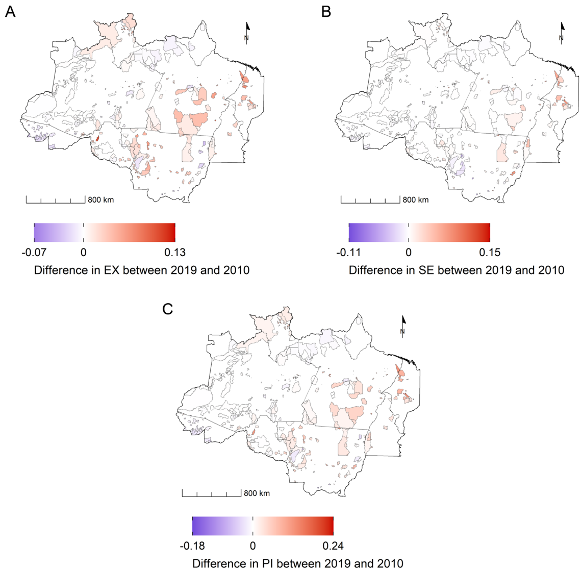
Figure 4.8 - The difference between the Exposure (A), Sensitivity (B), and Potential Impact (C) indexes between the periods 2001-2010 ( t1 ) and 2011-2019 ( t2 ) (i.e. difference = index t2 - index t1 ). Because of the lack of mining data available for the first period, mining was not considered in the calculation of these indexes. Negative values mean that the index is higher in period t1 , while positive values represent that the index is higher in period t2 .
