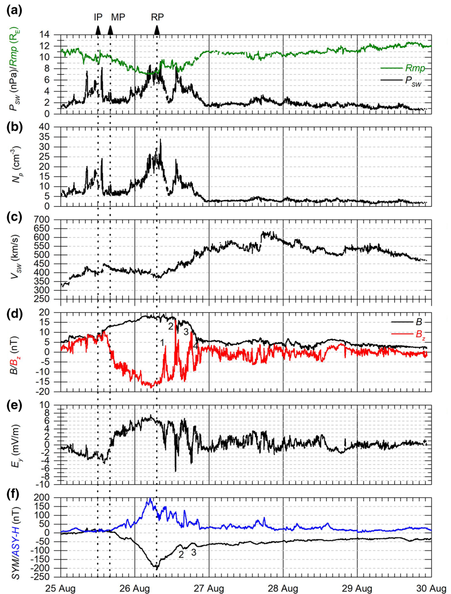
Figure 2. Interplanetary and geophysical parameters from August 25 to 29, 2018 geomagnetic storm: (a) solar wind pressure P_{sw} (black line) and magnetopause standoff distance R_{mp} (olive line), (b) solar wind proton density N_p , (c) solar wind speed V_{sw} , (d) IMF B (black line) and north-south IMF B_z component (red line) in GSM coordinate, (e) estimated dawn to dusk IEF E_y component, and (f) asymmetric ring current ASY-H (blue line) and symmetric ring current SYM-H (black line) indexes. The vertical dotted lines and labels indicate the initial (IP; 12:00 UT), main (MP; 16:00 UT), and recovery (RP; 7:00 UT) phases of the geomagnetic storm, respectively.
