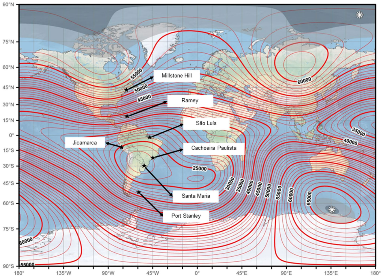
Figure 1. Global map with the geomagnetic field total intensity. The South American Magnetic Anomaly (SAMA) position is defined by the lowest iso-intensity line (23,000 nT) currently located in South America. The contour interval is 1,000 nT. The map also shows the different ionosonde stations used in this work. Source: Modified from Chulliat et al. (2020).
