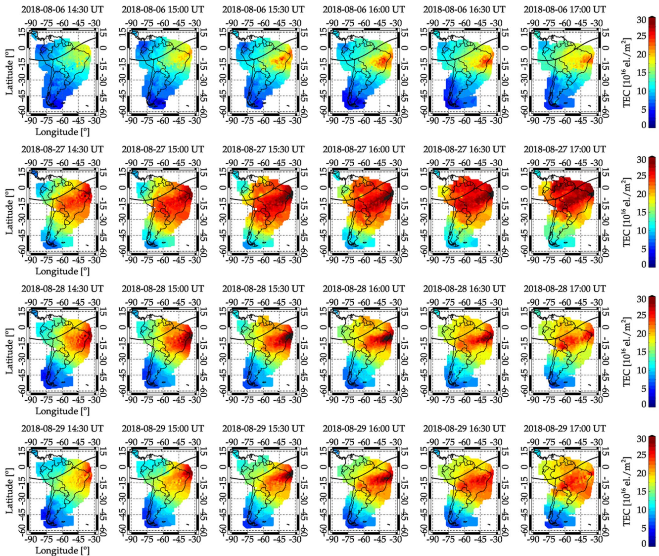
Figure 8. Sequence of TEC maps over South America from 14:30 UT to 17:00 UT on the quiet day of August 6, 2018 (first row) and during the August 27, 28, and 29, 2018 (second, third, and fourth row, respectively). The color scale indicates the TEC intensity. The curved solid line in each map is the geomagnetic equator. TEC, total electron content.
