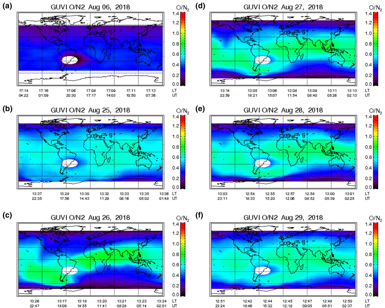
Figure 7. Global maps of the thermospheric [O]/[N_2] ratio derived from TIMED/GUVI (a) on the quiet day of August 6, 2018 and (b–f) during the August 25–29, 2018 geomagnetic storm. GUVI, Global ultraviolet imager; TIMED, Thermosphere Ionosphere Mesosphere Energetics and Dynamics.
