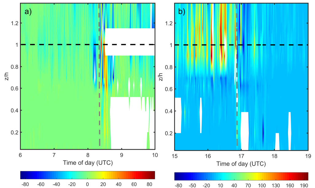
Figure 6. Temporal variation of the vertical profile of the sensible heat flux, H , ( \text{W m}^{-2} ), on 21 April 2014, measured at site T0k, during the passage of branch 1 (a) and branch 2 (b) of the SL2. The dashed black line indicates the forest canopy-top height. The dashed gray line indicates the arrival time of the downdrafts near the top of the forest trees.
