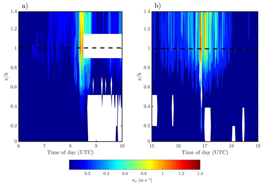
Figure 5. Temporal variation of the vertical profile of \sigma_w [ \text{m s}^{-1} ] on 21 April 2014 measured at site T0k during: (a) the passage of branch 1, and (b) of the branch 2 of SL2. The dashed black line corresponds to the top of the canopy. The white rectangle indicates the absence of data.
