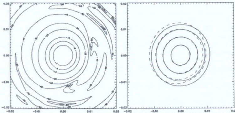
Fig. 5. Contour plot in the (u,v) plane of the main beam at 30 GHz of the channel F (left) and the Gaussian elliptical fit of the same beam (right). The dashed lines are the contour plot of the beam superimposed to the contour plot of the fitting function.
