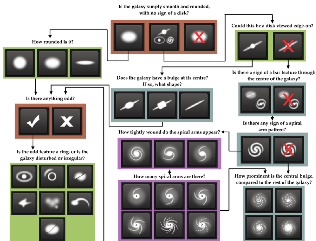
Figure 2.3 - Galaxy Zoo 2.
