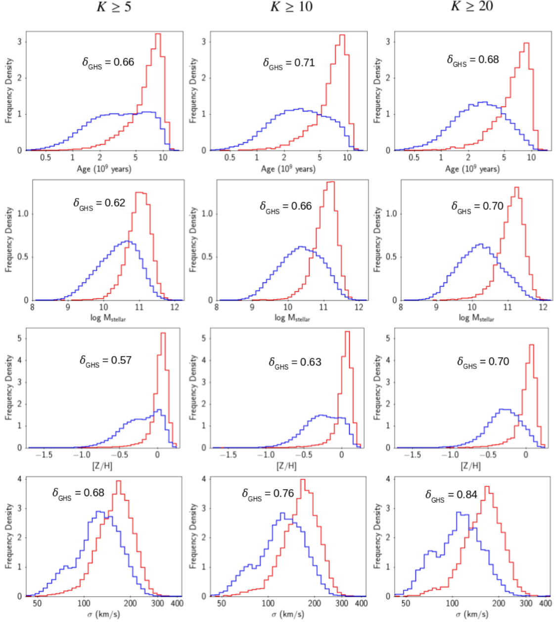
Figure 4.9 - Spectroscopic validation.
