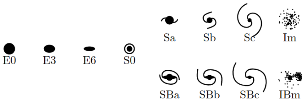
Figure 2.1 - Hubble sequence of galaxy morphologies.
