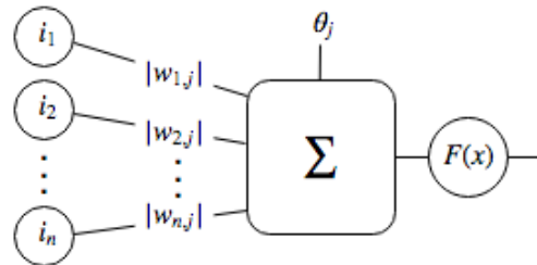
Figure 2.4 - Schematic representation of a neuron.
