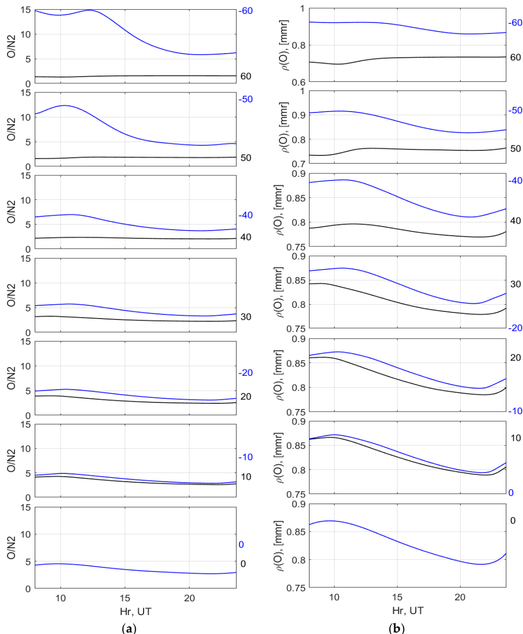
Figure 13. TIEGCM-simulated O/N 2 ratio (a) and O (b) at a fixed longitude of 65° W. The blue line represents the O and O/N 2 ratio in the southern hemisphere (SH). The black lines represent the O and O/N 2 ratio in the northern hemisphere (NH).
