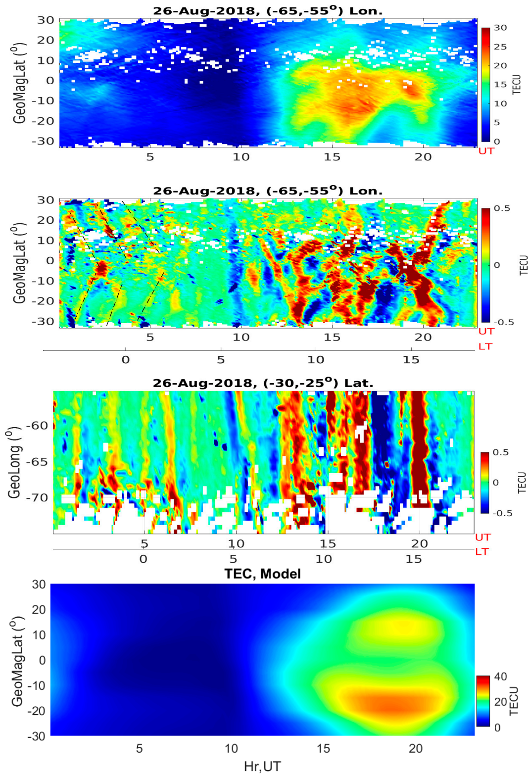
Figure 7. From top to bottom: keogram of background GNSS-TEC, keogram of TID obtained by removing the background TEC as a function of latitude and local and universal time, a keogram of TID as a function of longitude and local and universal time on 26 August 2018, and the simulation of TEC using the TIEGCM (at \pm 30^\circ geomagnetic latitudes).
