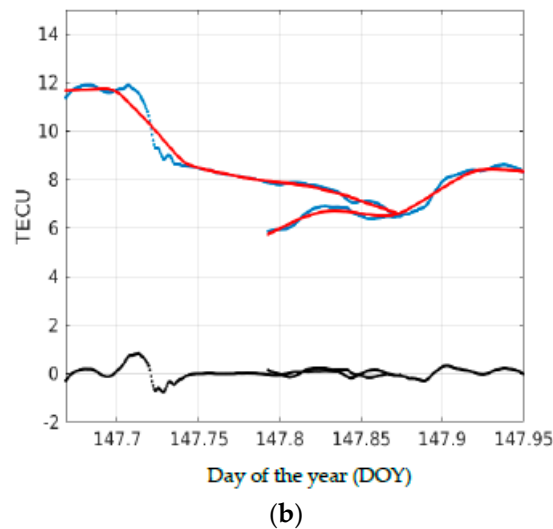
Figure 1. (a) An example of ionospheric pierce point distribution of the total electron content (TEC) measurement on 8 May 2017 at 10:00 UT. The black line represents the magnetic equator. (b) Examples of traveling ionospheric disturbances (TID) analysis procedures. The blue line represents the background TEC from one station and two satellites, the red line represents the hourly sliding window using the Savitzky–Golay low-pass filter, and the black line represents the differential TEC ( \Delta TEC).
