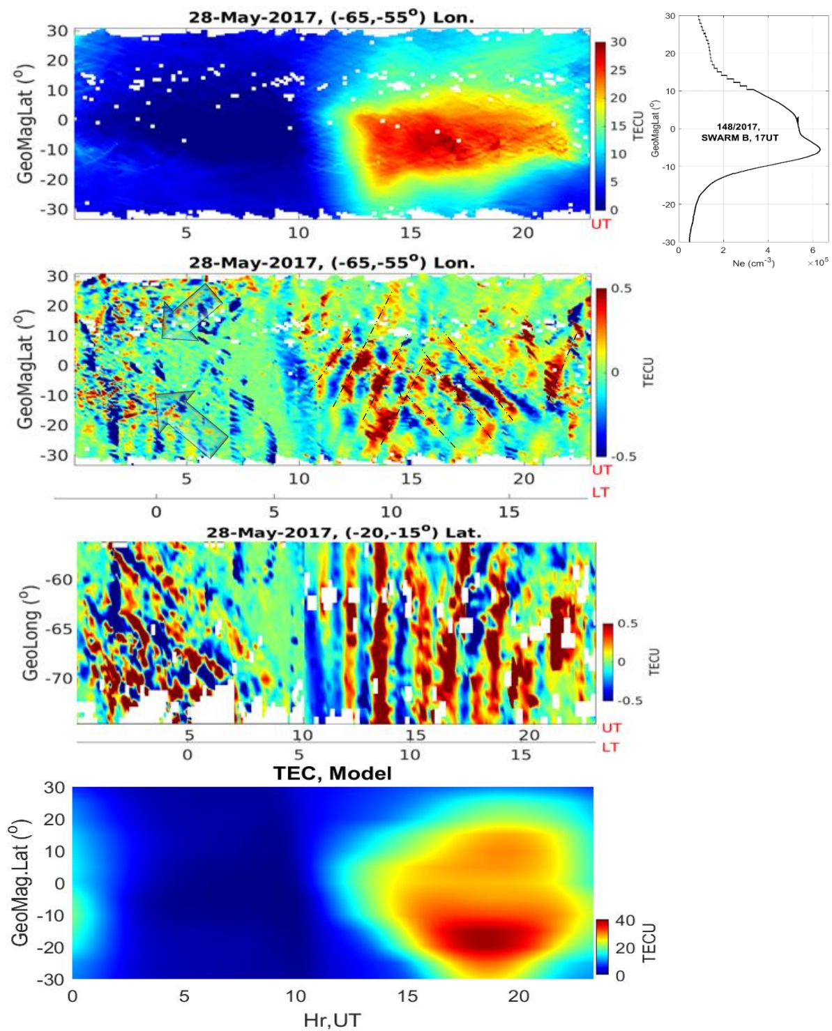
Figure 3. From top to bottom: keogram of background GNSS-TEC; on the right is the electron density obtained from the SWARM B satellite; keogram of TID obtained by removing the background TEC as a function of latitude and local and universal time (longitude: 55–65° S); keogram of TID as a function of longitude, local, and universal time on 28 May 2017; and the simulation of TEC using the thermosphere–ionosphere–electrodynamics general circulation model (TIEGCM) (at ±30° geomagnetic latitudes).
