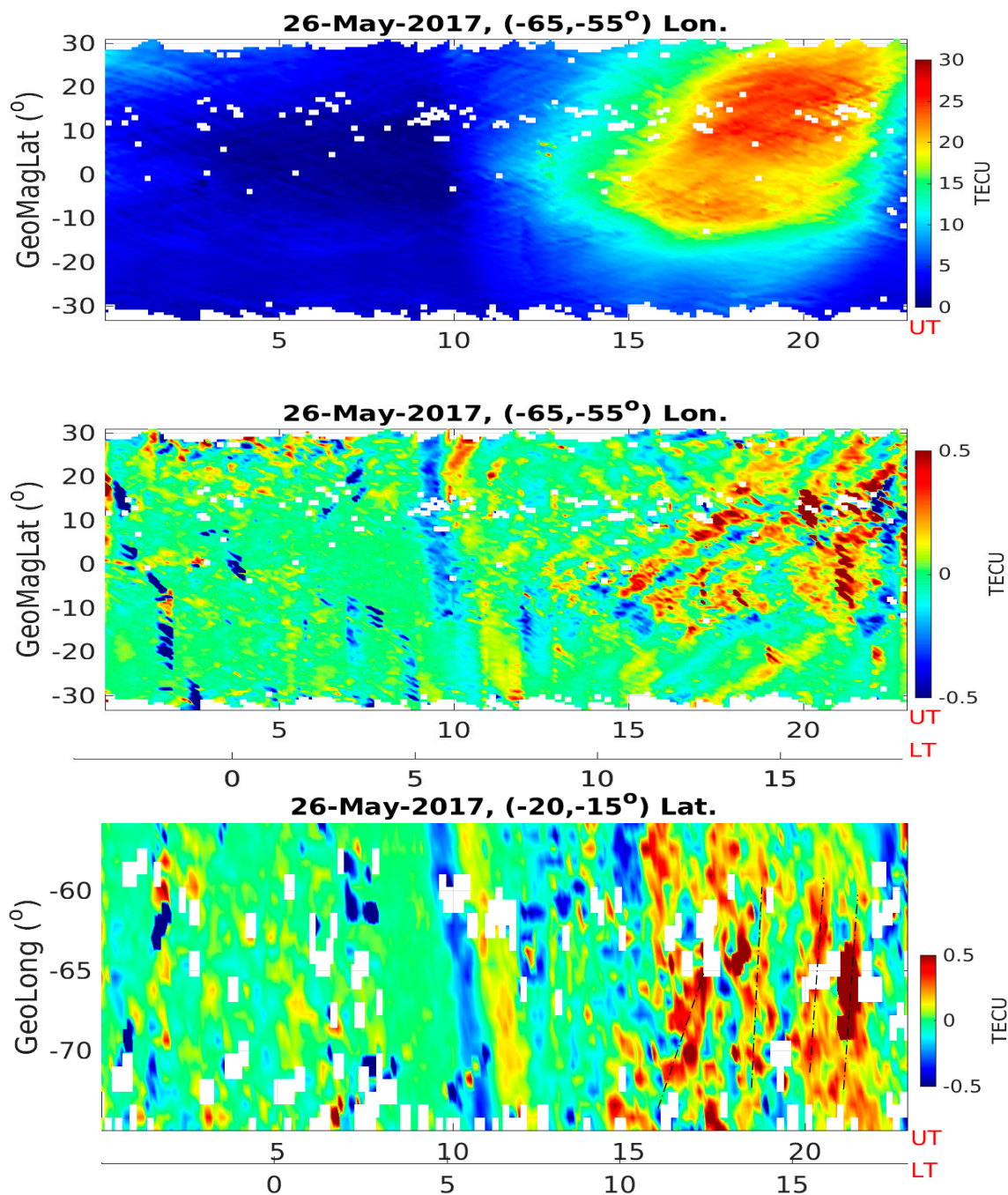
Figure 5. The same plots as Figure 3, but for a quiet day: 26 May 2017. The dashed lines on the bottom panel are determined by tracking the pack to pack of each wave using visual assessment.
