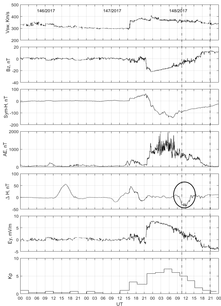
Figure 2. Geophysical and geomagnetic conditions during 26–28 May 2017. From top to bottom: solar wind speed ( V_{sw} ), the B_z component of the magnetic field of interplanetary magnetic field (IMF), the symmetric magnetic field strength (Sym-H) index, the auroral electrojet (AE) index, \Delta H_{(Belem - Petrolina)} , interplanetary east–west electric field ( E_y , positive to east), and the K_p magnetic index. The dashed lines represent the time period when different features of TIDs were observed. The black circle (on the \Delta H panel) highlights the \Delta H downward plasma drift on 28 May 2017.
