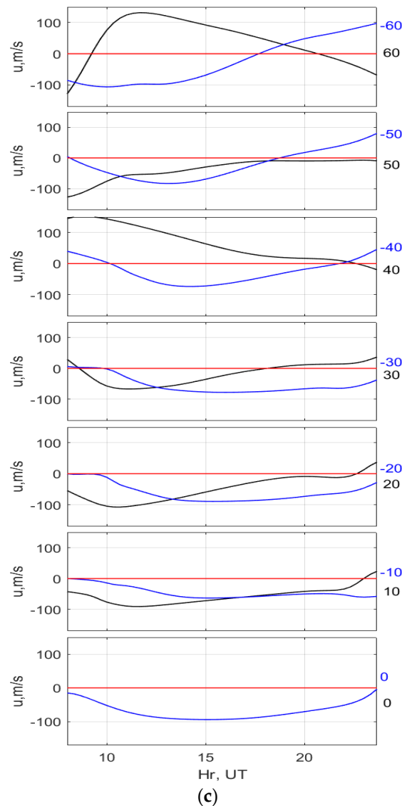
Figure 12. (a) Contour map for the meridional positive northward wind for both disturbed (top panel) and quiet (bottom panel) days. (b) TIEGCM result for 28 May 2017, showing meridional wind velocity changing from northward to southward geographically. (c) Same as (b) but in the magnetic meridian coordinate. The blue line represents the component of the wind in the south (0 to -60 degrees), and the black line represents the component of the winds in the north (0 to 60 degrees). The positive value of the winds indicates northward.
