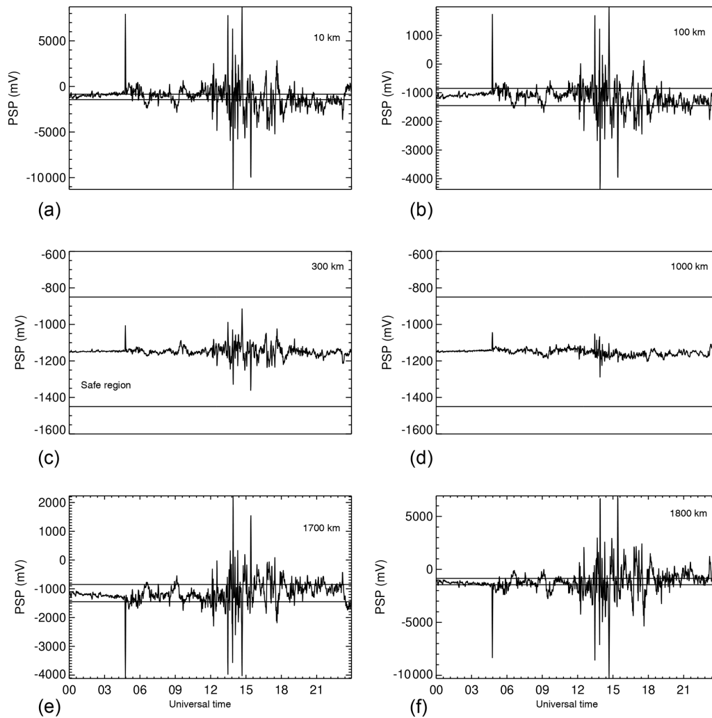
Figure 4. Pipe-to-soil potential obtained by DSLT theory for different sites (values in km at the top right of each panel) along the GASBOL pipeline for a terminating impedance of 1000 \Omega during the 17 March 2015 geomagnetic storm. Solid lines delimit the safe range of the GASBOL operation.
