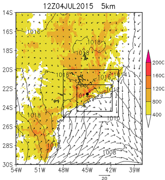
Figure 4 - Sea level pressure (contours in hPa) and surface wind ( \text{m s}^{-1} ) as simulated by the Eta-5 valid for 4 July 2015 at 12 UTC (24-h simulation) and terrain elevation (colors bar in meters above sea level). The outer box encompasses the area covered in next figures. The inner box encompasses the area of the Eta-1 domain used later. The black dot within the inner box shows the location of Cruzeiro city.
