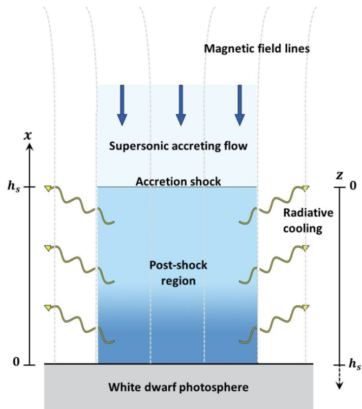
Figure 1.7 - The illustration of the accretion column. The PSR is produced when the accretion flow coming from the threading region reaches supersonic velocities. In the PSR, radiation processes cool matter and shape the density and the temperature profiles.
