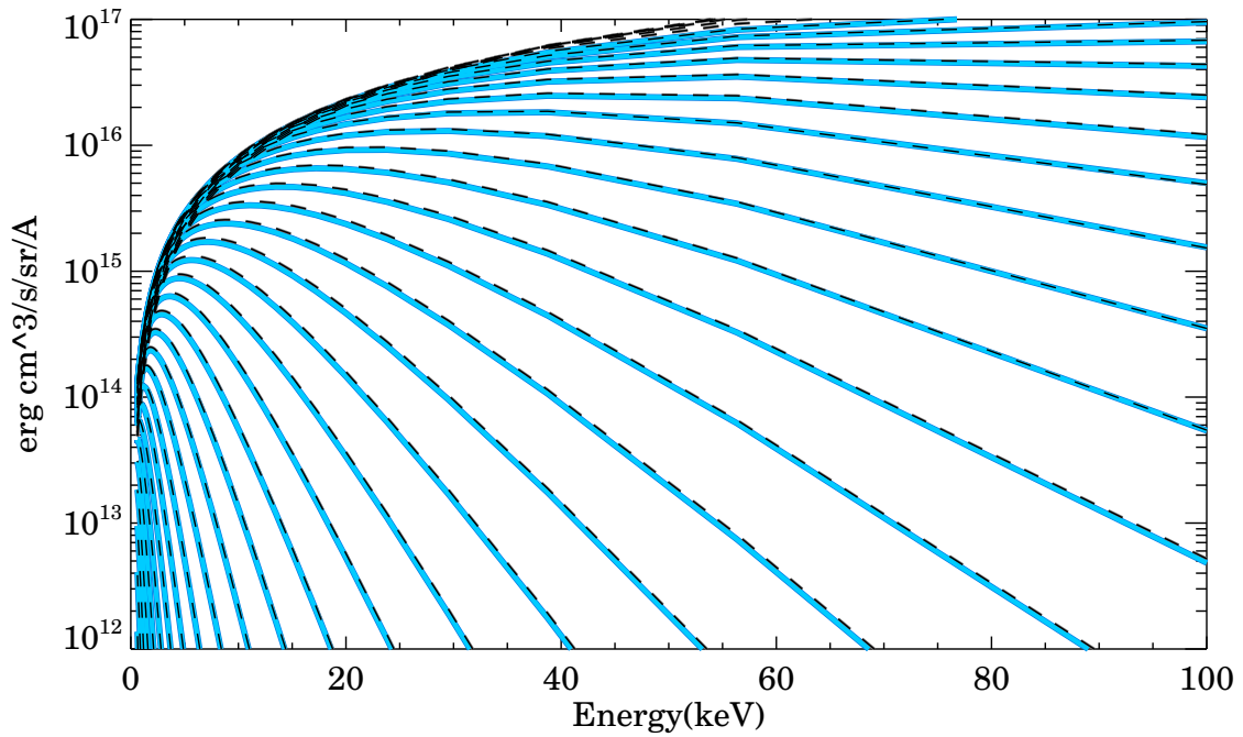
Figure 3.5 - Comparison of Gaunt factor of Mewe et al. (1986a) from CYCLOPS (blue continuous line and Sutherland (1998) and Itoh et al. (2000) (black dashed lines).
